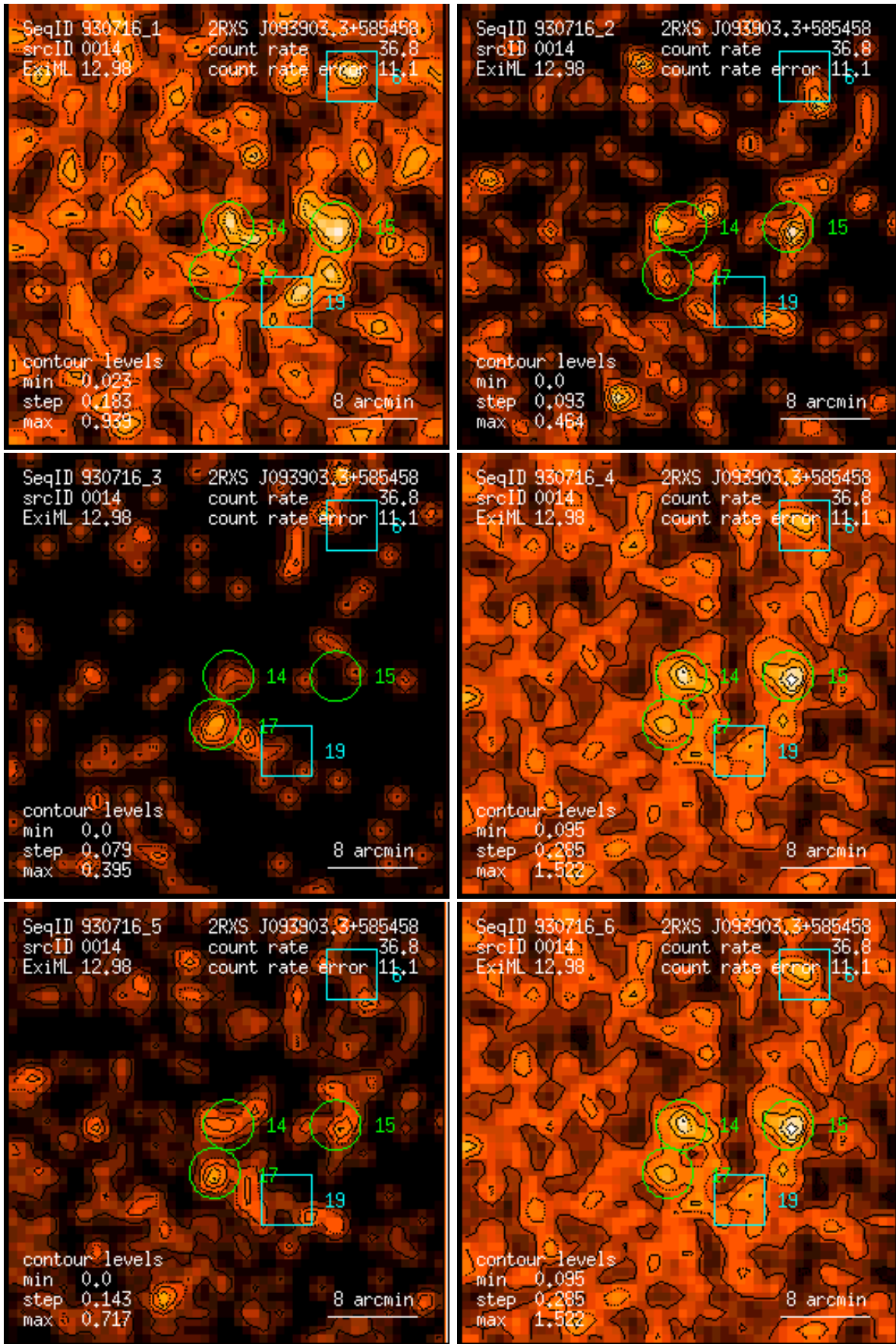
Figure 14: RASS 930716: detection 0014: band rate images, Gaussian filter: (1) PSPC channels 11 – 41, (2) 52 – 90, (3) 91 – 201, (4) 11 – 235, (5) 52 – 201, (6) 11 – 201. Broad band rates in counts/ks. Band rate contour levels in counts/ks/arcmin 2 .
