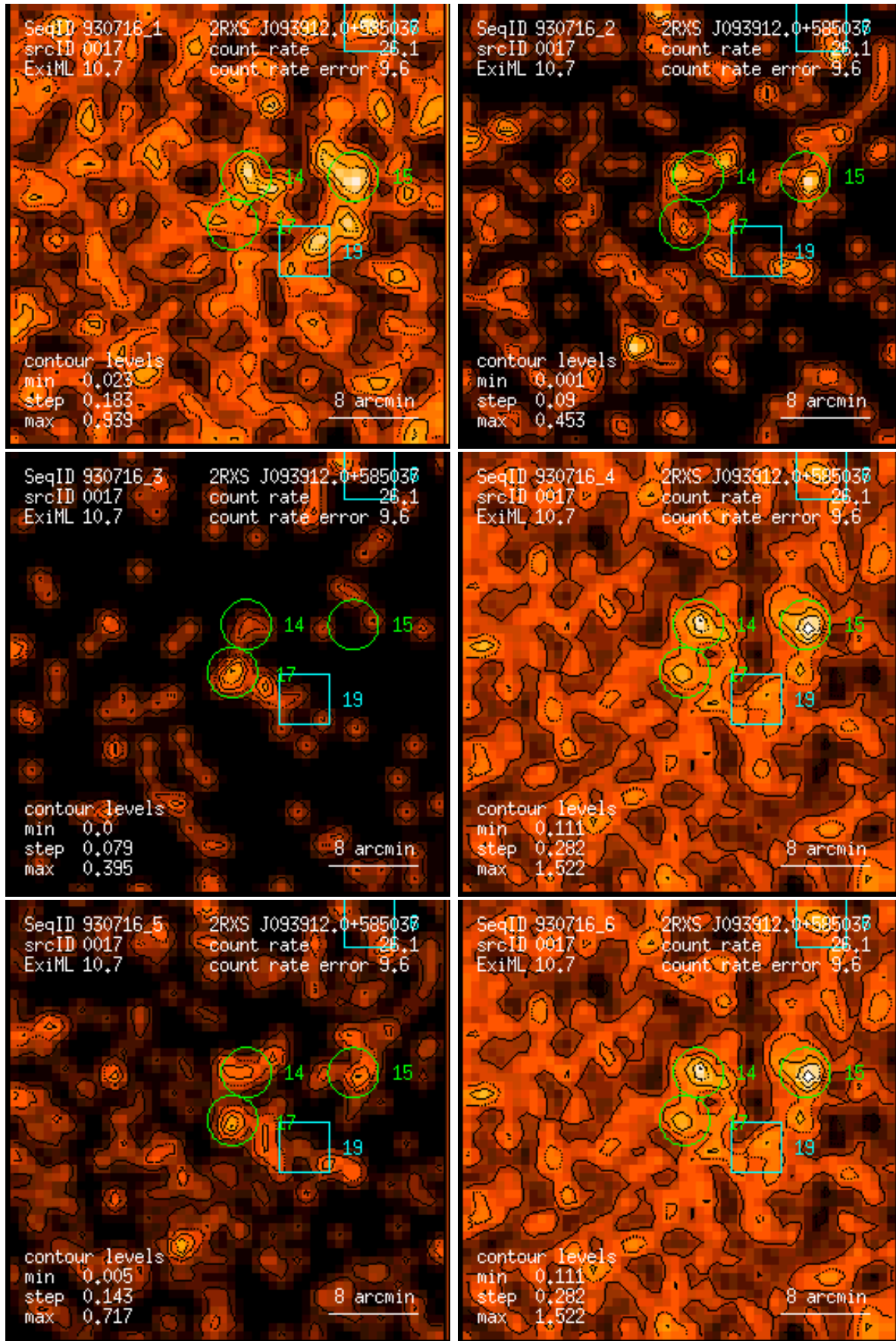
Figure 17: RASS 930716: detection 0017: band rate images, Gaussian filter: (1) PSPC channels 11 – 41, (2) 52 – 90, (3) 91 – 201, (4) 11 – 235, (5) 52 – 201, (6) 11 – 201. Broad band rates in counts/ks. Band rate contour levels in counts/ks/arcmin 2 .
