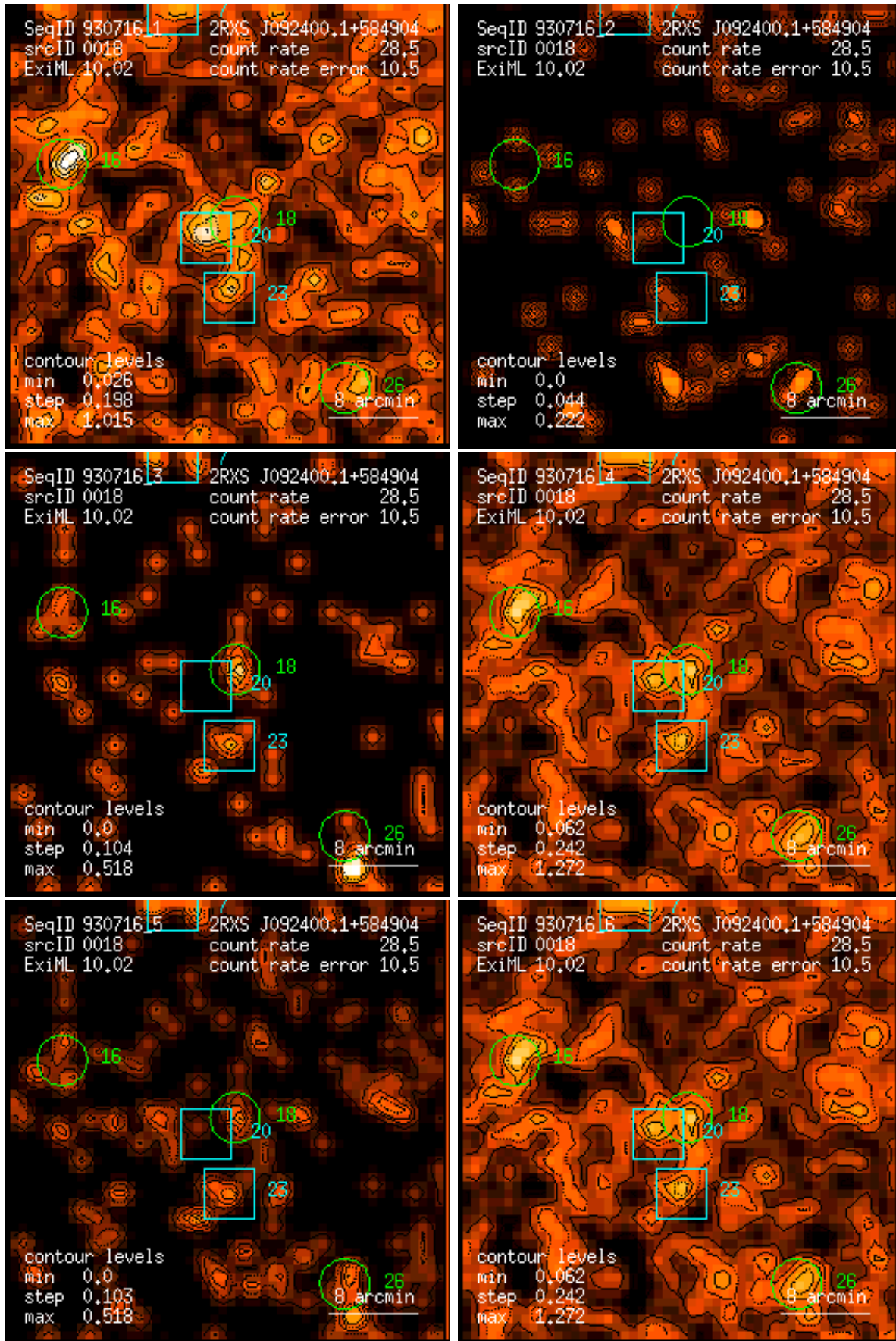
Figure 18: RASS 930716: detection 0018: band rate images, Gaussian filter: (1) PSPC channels 11 – 41, (2) 52 – 90, (3) 91 – 201, (4) 11 – 235, (5) 52 – 201, (6) 11 – 201. Broad band rates in counts/ks. Band rate contour levels in counts/ks/arcmin 2 .
