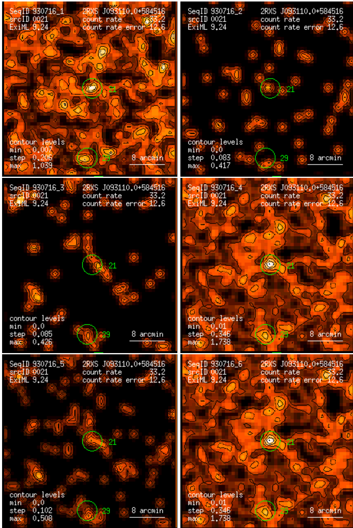
Figure 21: RASS 930716: detection 0021: band rate images, Gaussian filter: (1) PSPC channels 11 – 41, (2) 52 – 90, (3) 91 – 201, (4) 11 – 235, (5) 52 – 201, (6) 11 – 201. Broad band rates in counts/ks. Band rate contour levels in counts/ks/arcmin 2 .
