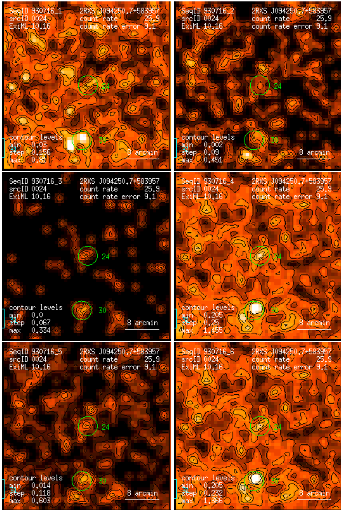
Figure 24: RASS 930716: detection 0024: band rate images, Gaussian filter: (1) PSPC channels 11 – 41, (2) 52 – 90, (3) 91 – 201, (4) 11 – 235, (5) 52 – 201, (6) 11 – 201. Broad band rates in counts/ks. Band rate contour levels in counts/ks/arcmin 2 .
