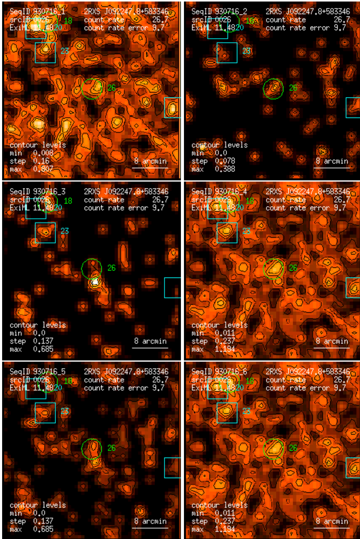
Figure 26: RASS 930716: detection 0026: band rate images, Gaussian filter: (1) PSPC channels 11 – 41, (2) 52 – 90, (3) 91 – 201, (4) 11 – 235, (5) 52 – 201, (6) 11 – 201. Broad band rates in counts/ks. Band rate contour levels in counts/ks/arcmin 2 .
