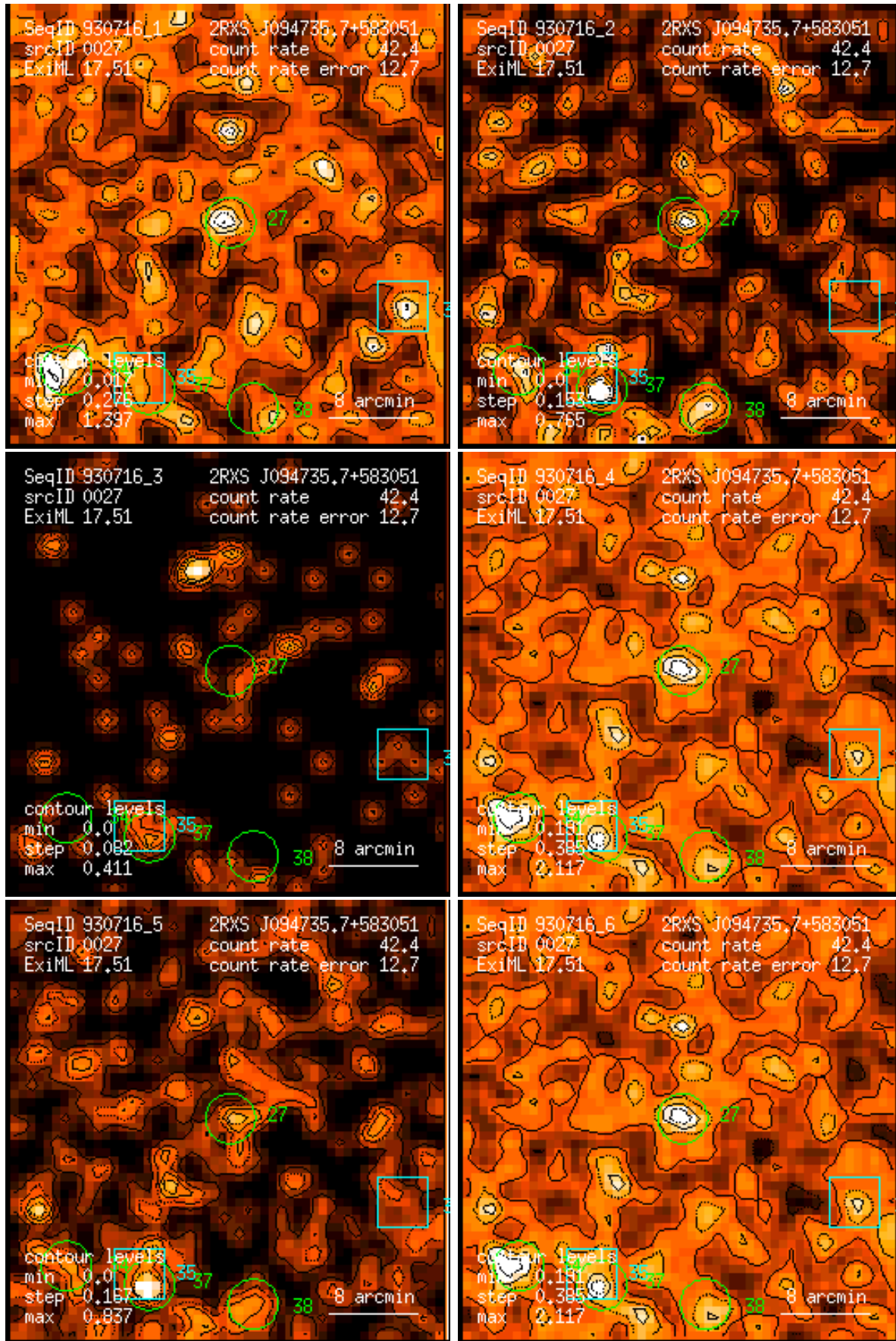
Figure 27: RASS 930716: detection 0027: band rate images, Gaussian filter: (1) PSPC channels 11 – 41, (2) 52 – 90, (3) 91 – 201, (4) 11 – 235, (5) 52 – 201, (6) 11 – 201. Broad band rates in counts/ks. Band rate contour levels in counts/ks/arcmin 2 .
