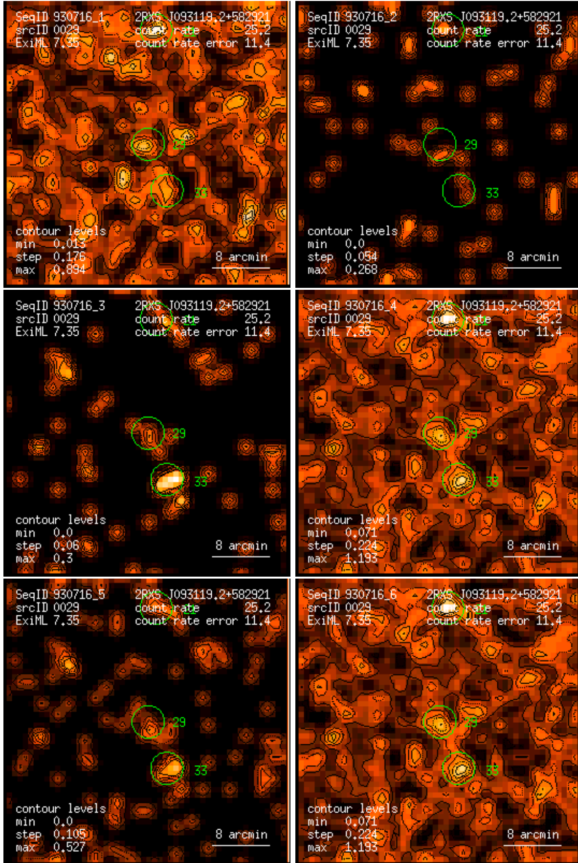
Figure 29: RASS 930716: detection 0029: band rate images, Gaussian filter: (1) PSPC channels 11 – 41, (2) 52 – 90, (3) 91 – 201, (4) 11 – 235, (5) 52 – 201, (6) 11 – 201. Broad band rates in counts/ks. Band rate contour levels in counts/ks/arcmin 2 .
