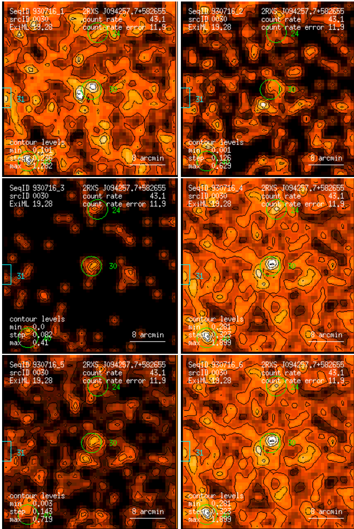
Figure 30: RASS 930716: detection 0030: band rate images, Gaussian filter: (1) PSPC channels 11 – 41, (2) 52 – 90, (3) 91 – 201, (4) 11 – 235, (5) 52 – 201, (6) 11 – 201. Broad band rates in counts/ks. Band rate contour levels in counts/ks/arcmin 2 .
