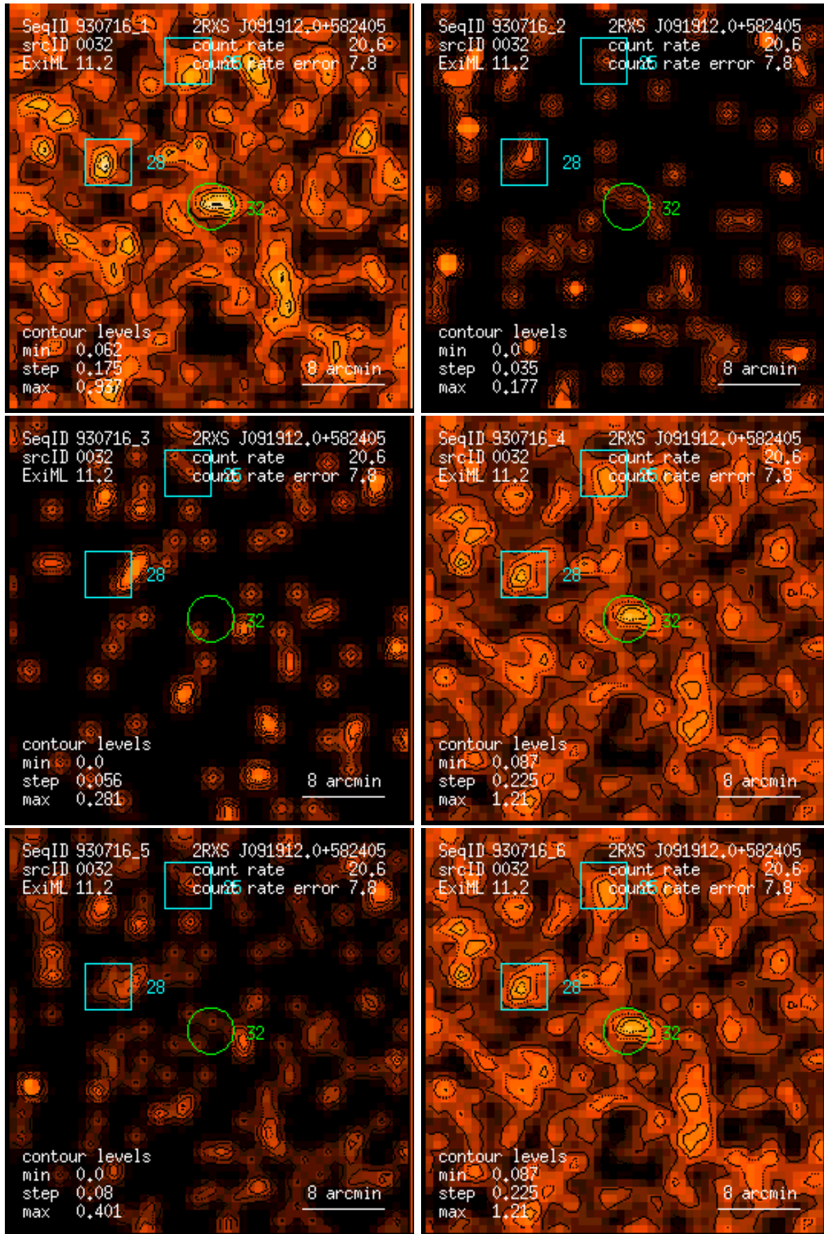
Figure 32: RASS 930716: detection 0032: band rate images, Gaussian filter: (1) PSPC channels 11 – 41, (2) 52 – 90, (3) 91 – 201, (4) 11 – 235, (5) 52 – 201, (6) 11 – 201. Broad band rates in counts/ks. Band rate contour levels in counts/ks/arcmin 2 .
