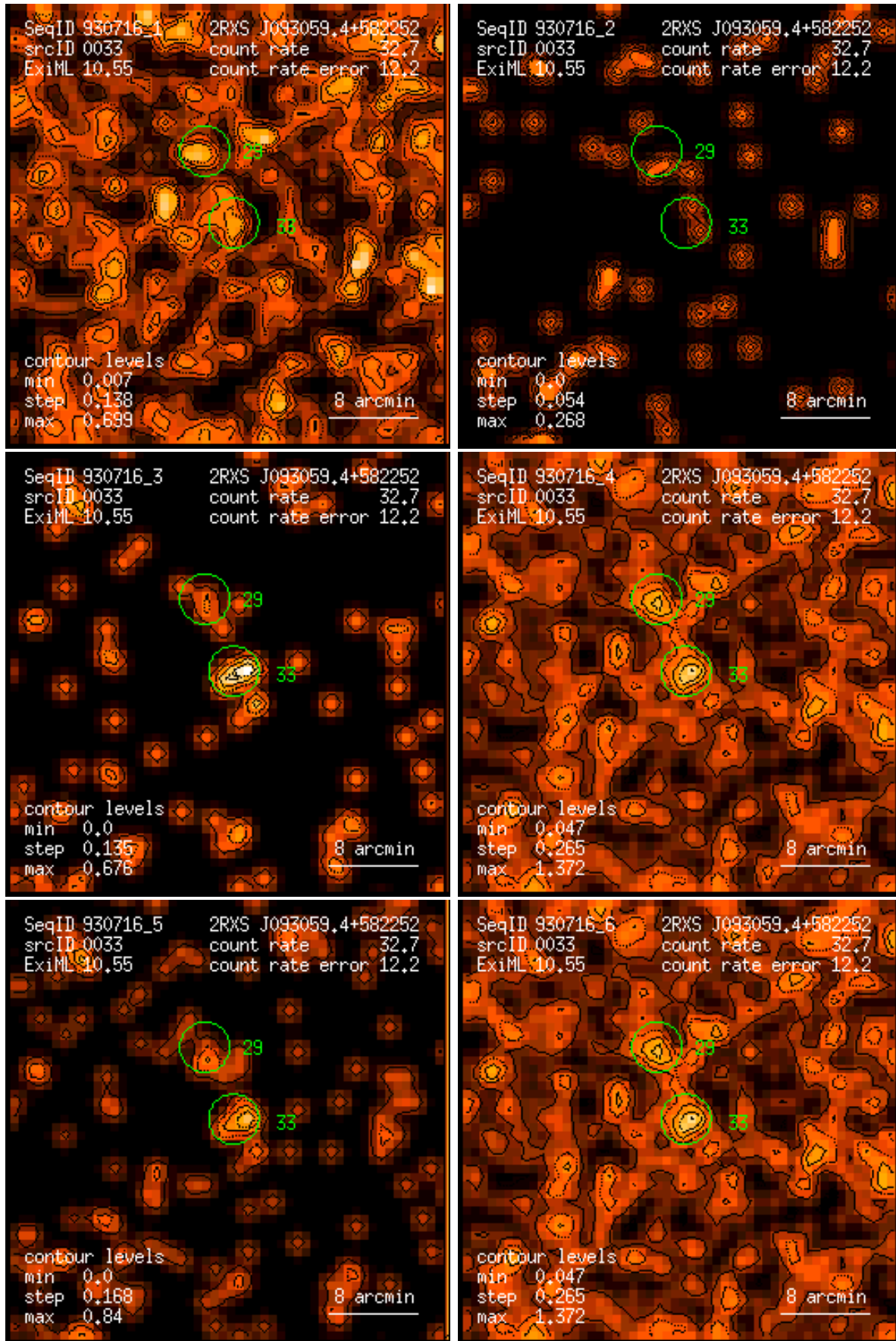
Figure 33: RASS 930716: detection 0033: band rate images, Gaussian filter: (1) PSPC channels 11 – 41, (2) 52 – 90, (3) 91 – 201, (4) 11 – 235, (5) 52 – 201, (6) 11 – 201. Broad band rates in counts/ks. Band rate contour levels in counts/ks/arcmin 2 .
