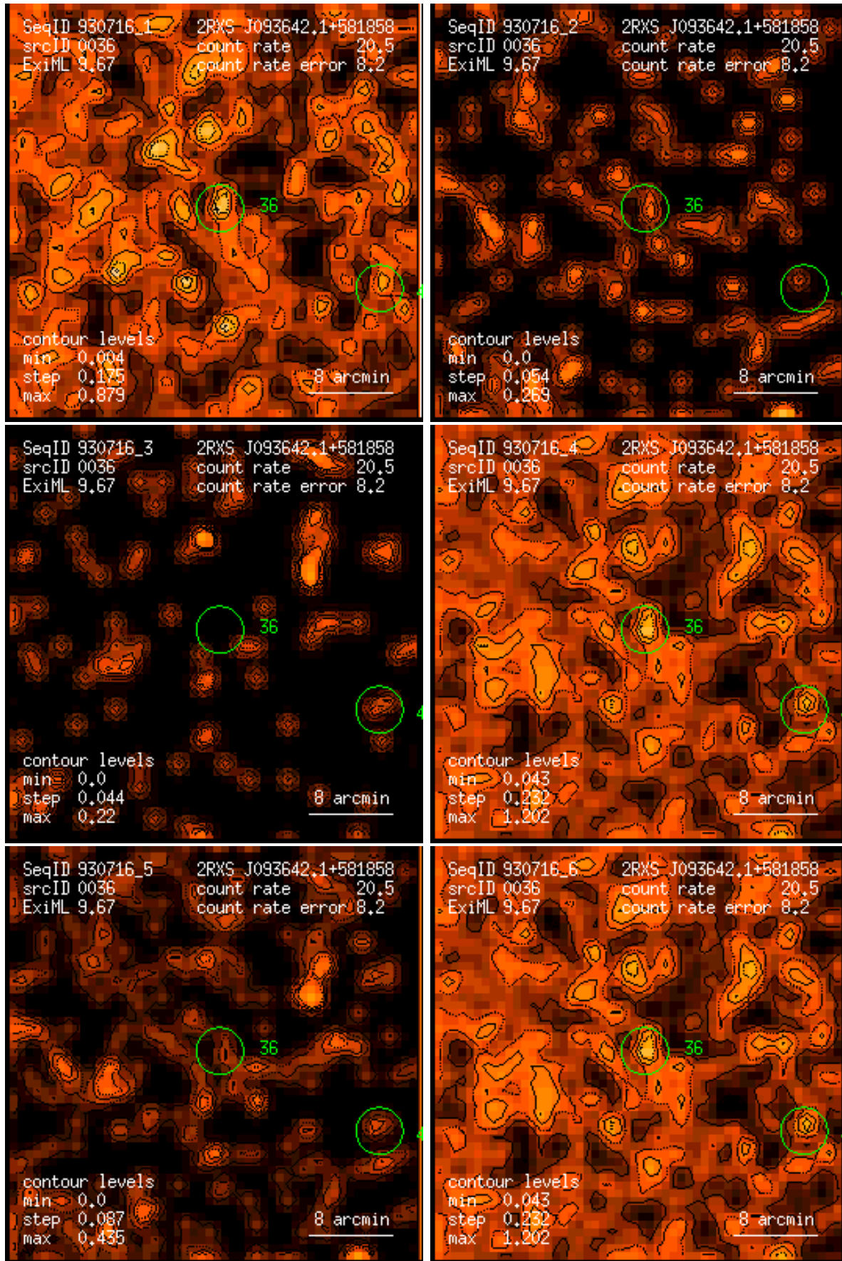
Figure 36: RASS 930716: detection 0036: band rate images, Gaussian filter: (1) PSPC channels 11 – 41, (2) 52 – 90, (3) 91 – 201, (4) 11 – 235, (5) 52 – 201, (6) 11 – 201. Broad band rates in counts/ks. Band rate contour levels in counts/ks/arcmin 2 .
