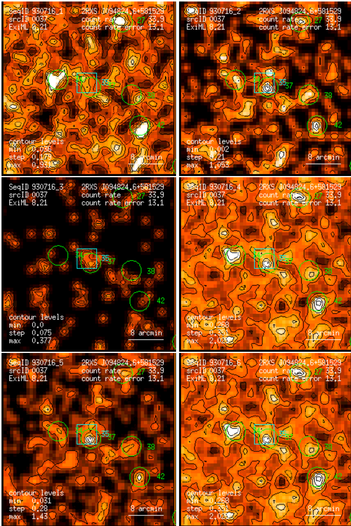
Figure 37: RASS 930716: detection 0037: band rate images, Gaussian filter: (1) PSPC channels 11 – 41, (2) 52 – 90, (3) 91 – 201, (4) 11 – 235, (5) 52 – 201, (6) 11 – 201. Broad band rates in counts/ks. Band rate contour levels in counts/ks/arcmin 2 .
