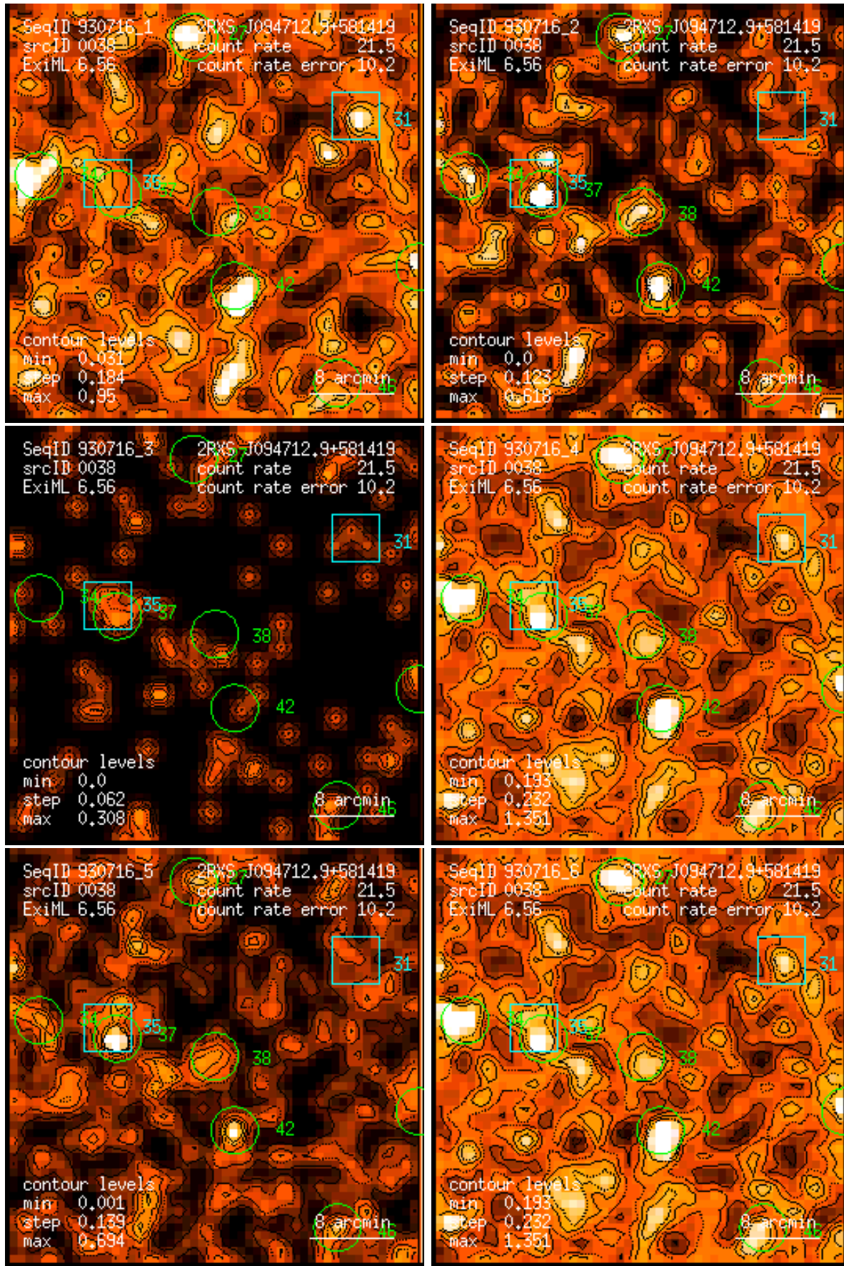
Figure 38: RASS 930716: detection 0038: band rate images, Gaussian filter: (1) PSPC channels 11 – 41, (2) 52 – 90, (3) 91 – 201, (4) 11 – 235, (5) 52 – 201, (6) 11 – 201. Broad band rates in counts/ks. Band rate contour levels in counts/ks/arcmin 2 .
