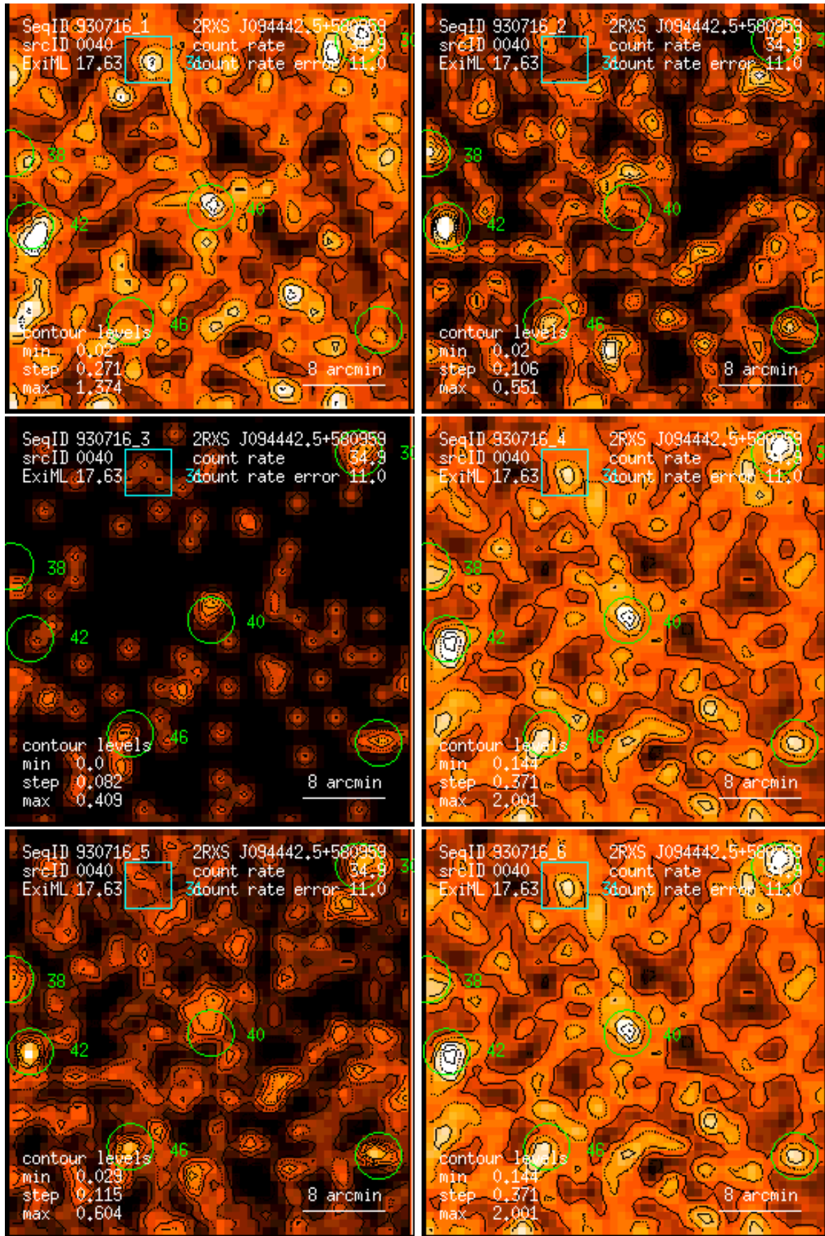
Figure 40: RASS 930716: detection 0040: band rate images, Gaussian filter: (1) PSPC channels 11 – 41, (2) 52 – 90, (3) 91 – 201, (4) 11 – 235, (5) 52 – 201, (6) 11 – 201. Broad band rates in counts/ks. Band rate contour levels in counts/ks/arcmin 2 .
