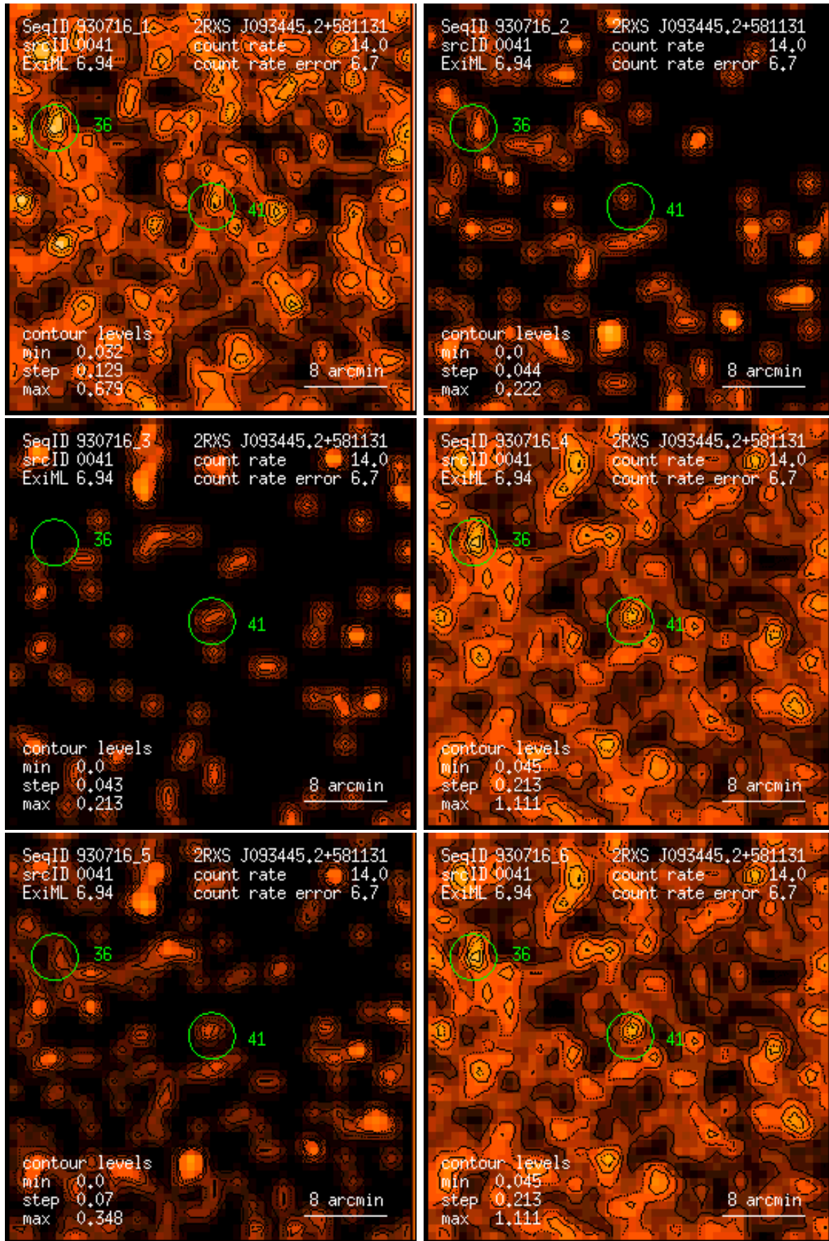
Figure 41: RASS 930716: detection 0041: band rate images, Gaussian filter: (1) PSPC channels 11 – 41, (2) 52 – 90, (3) 91 – 201, (4) 11 – 235, (5) 52 – 201, (6) 11 – 201. Broad band rates in counts/ks. Band rate contour levels in counts/ks/arcmin 2 .
