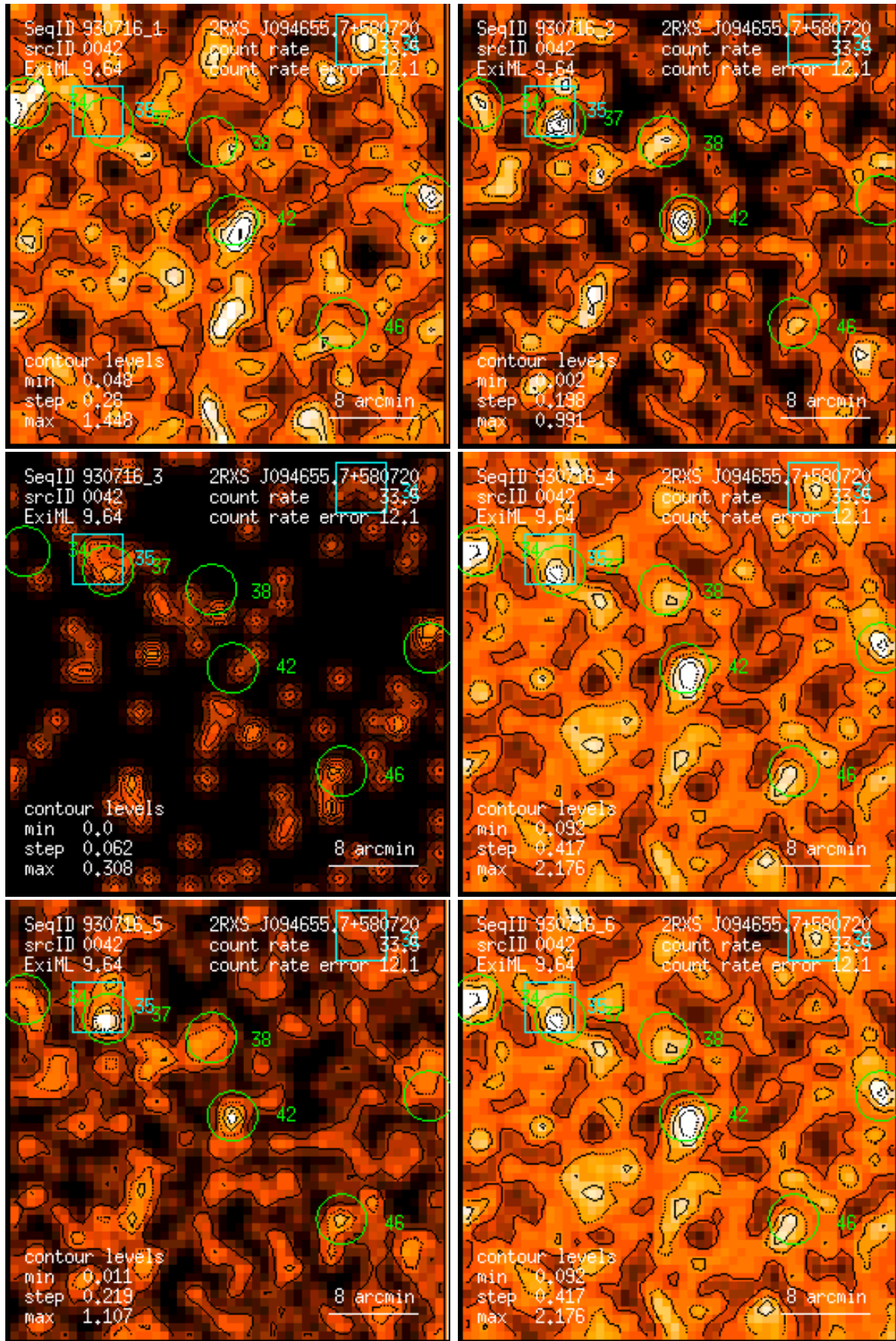
Figure 42: RASS 930716: detection 0042: band rate images, Gaussian filter: (1) PSPC channels 11 – 41, (2) 52 – 90, (3) 91 – 201, (4) 11 – 235, (5) 52 – 201, (6) 11 – 201. Broad band rates in counts/ks. Band rate contour levels in counts/ks/arcmin 2 .
