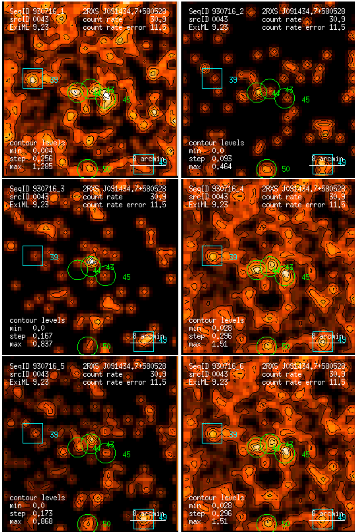
Figure 43: RASS 930716: detection 0043: band rate images, Gaussian filter: (1) PSPC channels 11 – 41, (2) 52 – 90, (3) 91 – 201, (4) 11 – 235, (5) 52 – 201, (6) 11 – 201. Broad band rates in counts/ks. Band rate contour levels in counts/ks/arcmin 2 .
