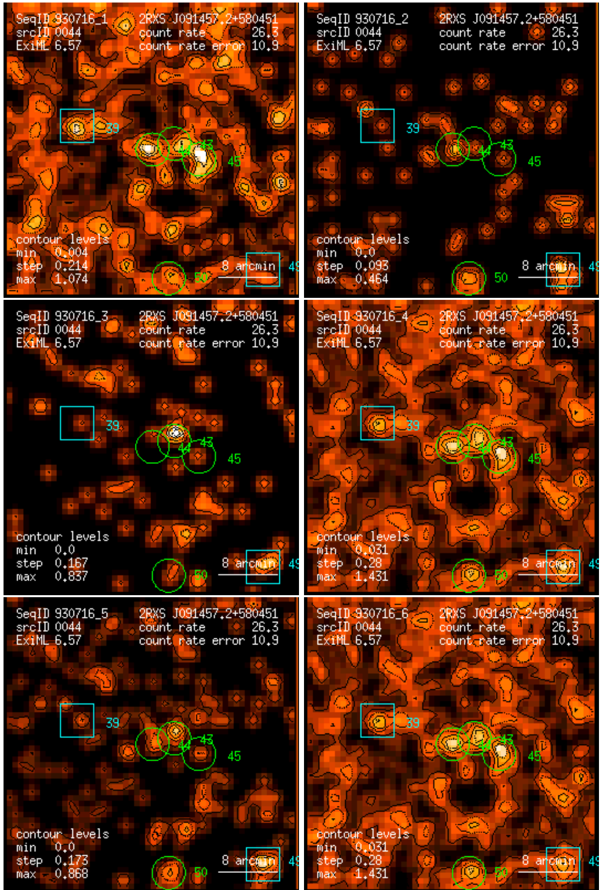
Figure 44: RASS 930716: detection 0044: band rate images, Gaussian filter: (1) PSPC channels 11 – 41, (2) 52 – 90, (3) 91 – 201, (4) 11 – 235, (5) 52 – 201, (6) 11 – 201. Broad band rates in counts/ks. Band rate contour levels in counts/ks/arcmin 2 .
