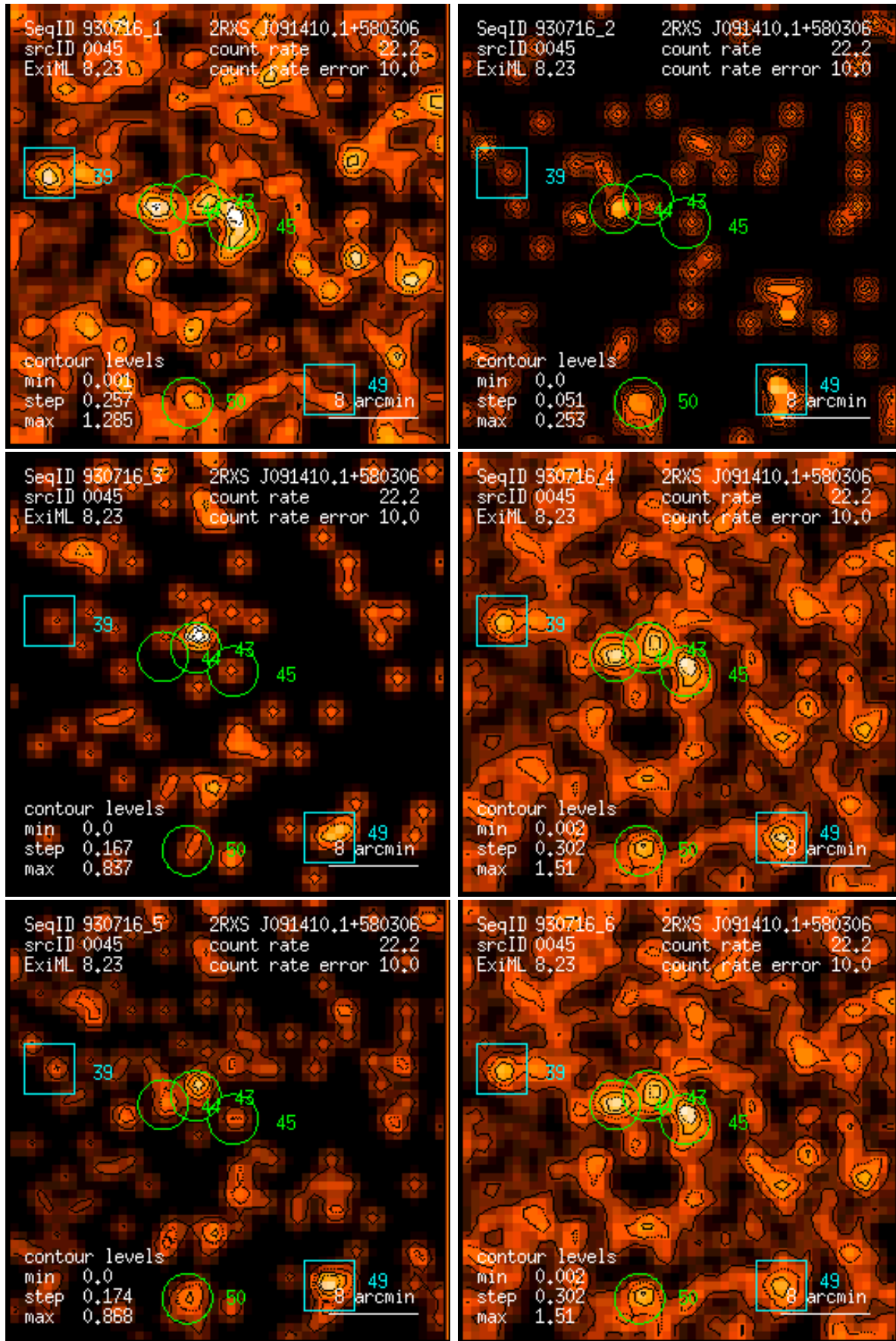
Figure 45: RASS 930716: detection 0045: band rate images, Gaussian filter: (1) PSPC channels 11 – 41, (2) 52 – 90, (3) 91 – 201, (4) 11 – 235, (5) 52 – 201, (6) 11 – 201. Broad band rates in counts/ks. Band rate contour levels in counts/ks/arcmin 2 .
