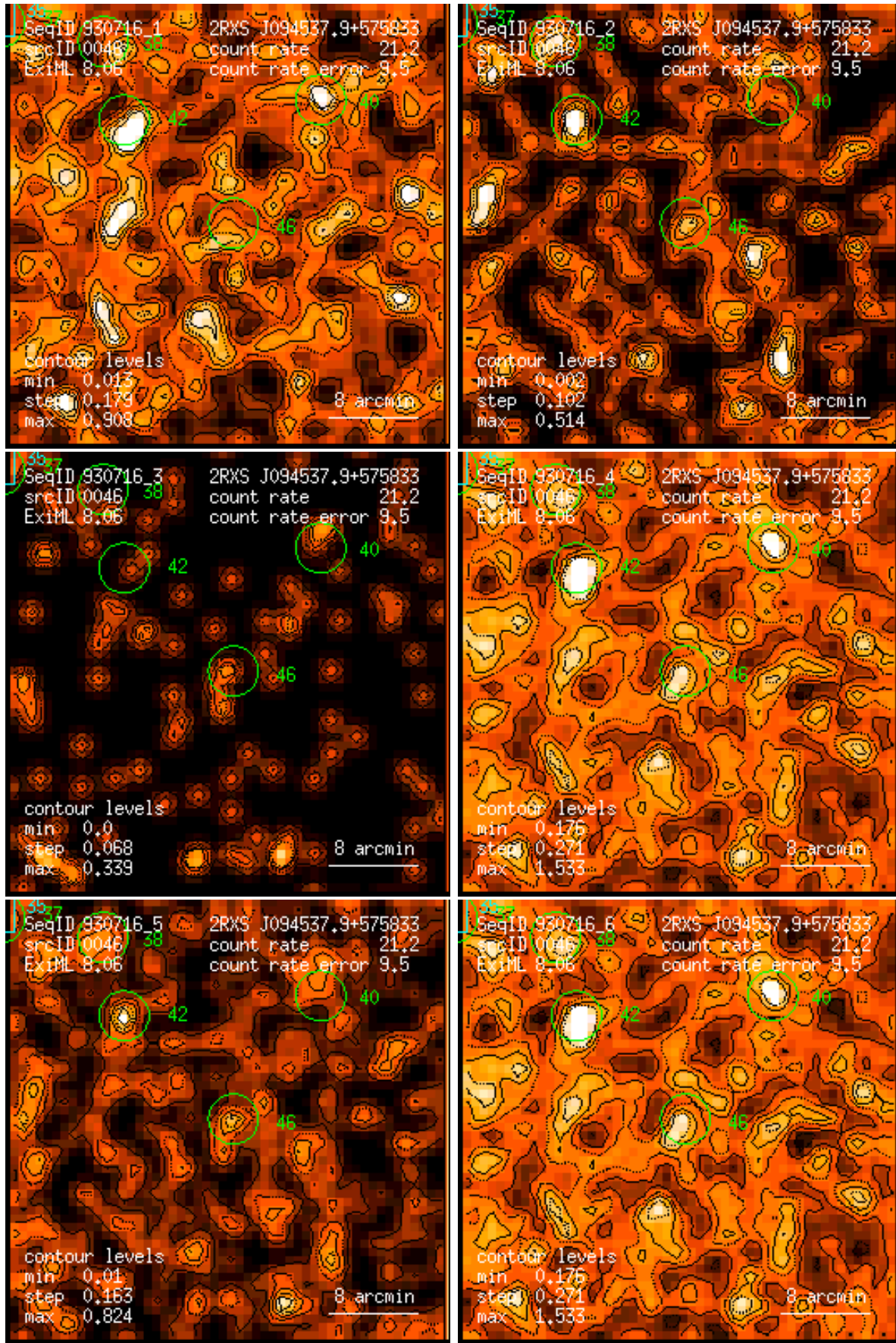
Figure 46: RASS 930716: detection 0046: band rate images, Gaussian filter: (1) PSPC channels 11 – 41, (2) 52 – 90, (3) 91 – 201, (4) 11 – 235, (5) 52 – 201, (6) 11 – 201. Broad band rates in counts/ks. Band rate contour levels in counts/ks/arcmin 2 .
