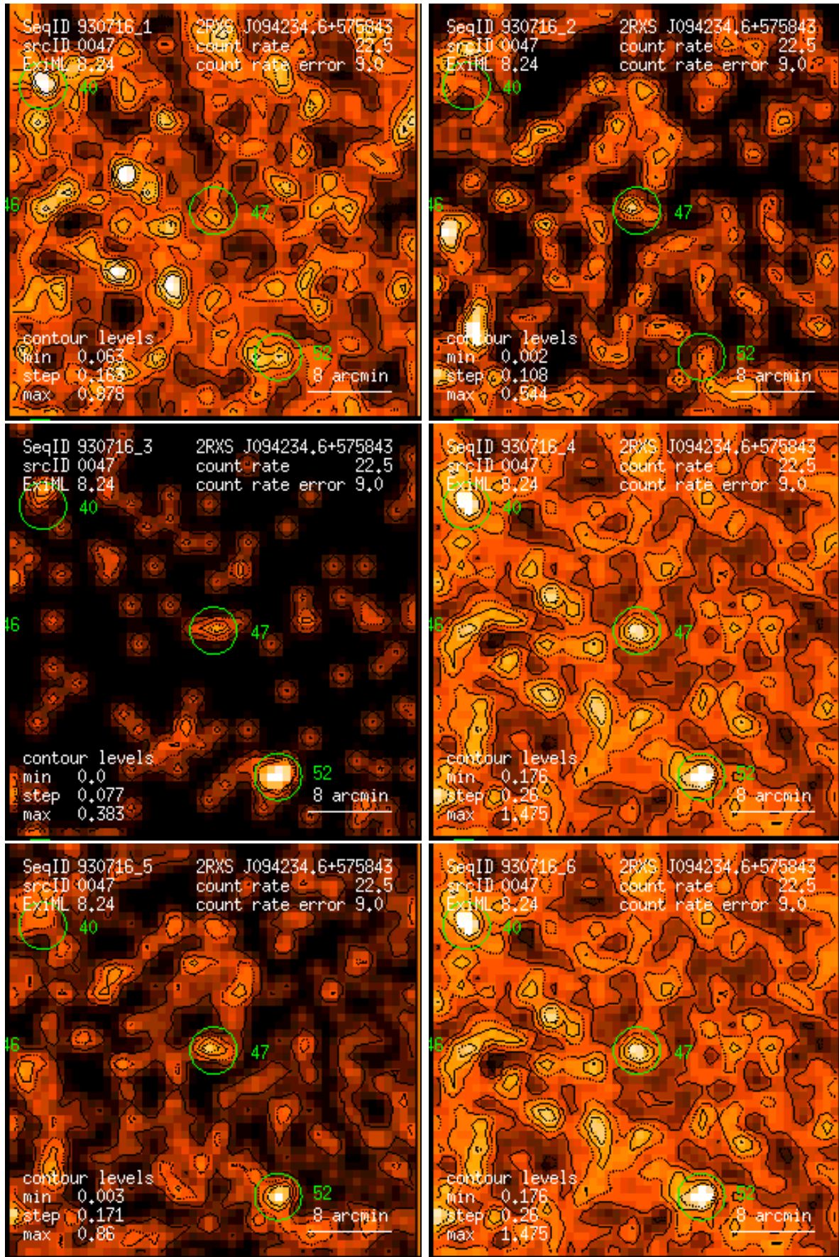
Figure 47: RASS 930716: detection 0047: band rate images, Gaussian filter: (1) PSPC channels 11 – 41, (2) 52 – 90, (3) 91 – 201, (4) 11 – 235, (5) 52 – 201, (6) 11 – 201. Broad band rates in counts/ks. Band rate contour levels in counts/ks/arcmin 2 .
