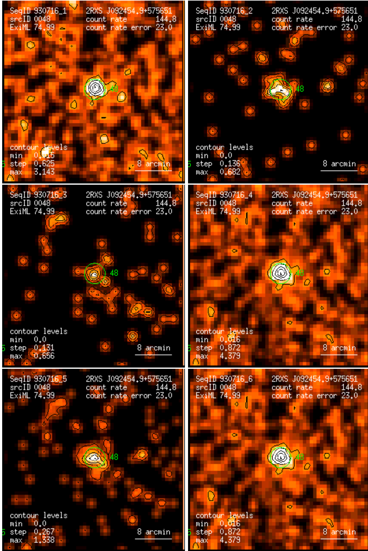
Figure 48: RASS 930716: detection 0048: band rate images, Gaussian filter: (1) PSPC channels 11 – 41, (2) 52 – 90, (3) 91 – 201, (4) 11 – 235, (5) 52 – 201, (6) 11 – 201. Broad band rates in counts/ks. Band rate contour levels in counts/ks/arcmin 2 .
