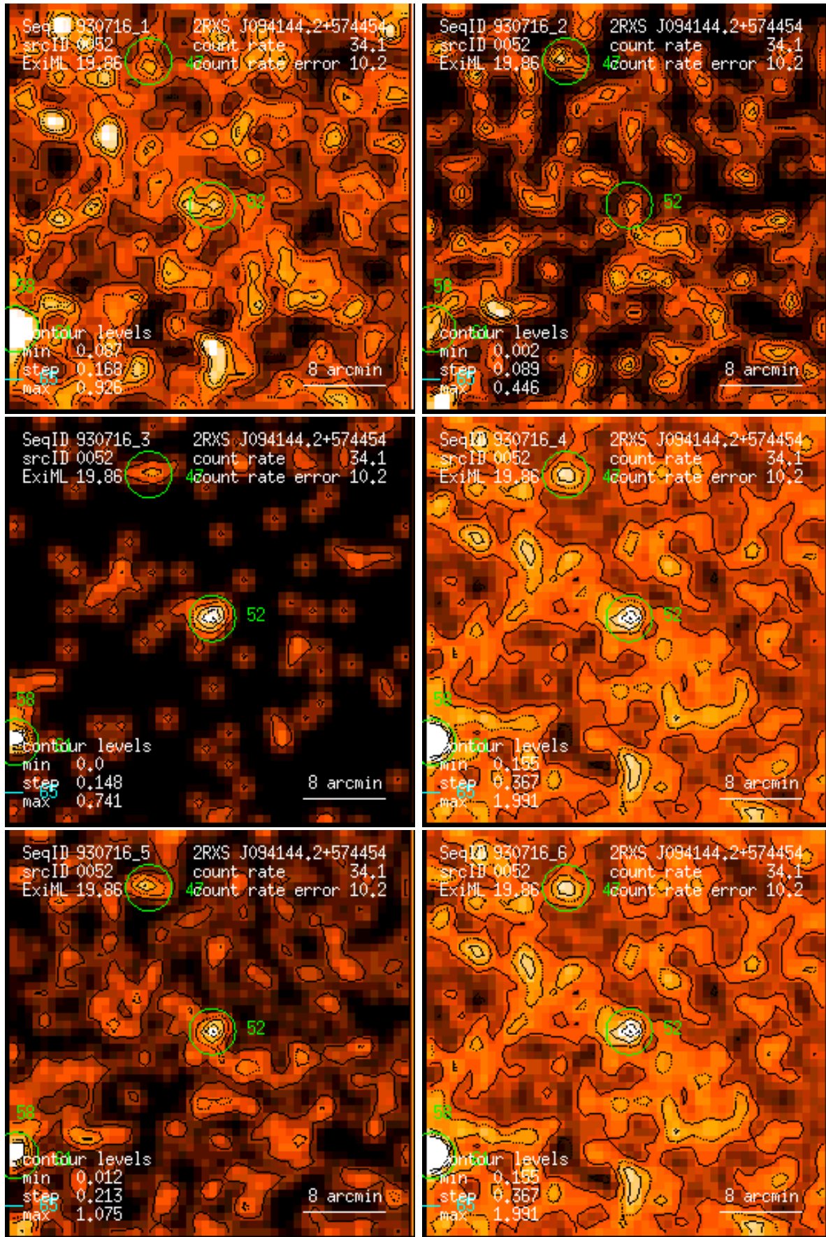
Figure 52: RASS 930716: detection 0052: band rate images, Gaussian filter: (1) PSPC channels 11 – 41, (2) 52 – 90, (3) 91 – 201, (4) 11 – 235, (5) 52 – 201, (6) 11 – 201. Broad band rates in counts/ks. Band rate contour levels in counts/ks/arcmin 2 .
