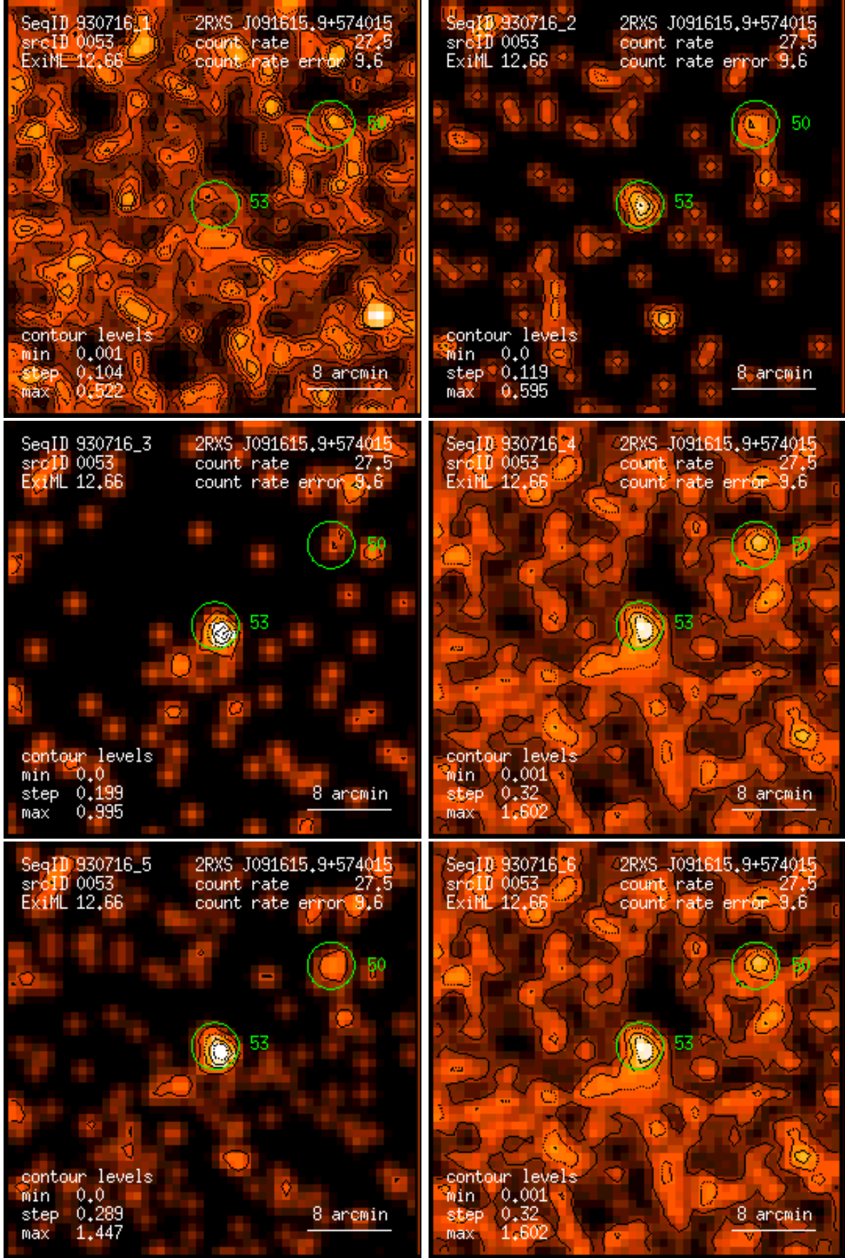
Figure 53: RASS 930716: detection 0053: band rate images, Gaussian filter: (1) PSPC channels 11 – 41, (2) 52 – 90, (3) 91 – 201, (4) 11 – 235, (5) 52 – 201, (6) 11 – 201. Broad band rates in counts/ks. Band rate contour levels in counts/ks/arcmin 2 .
