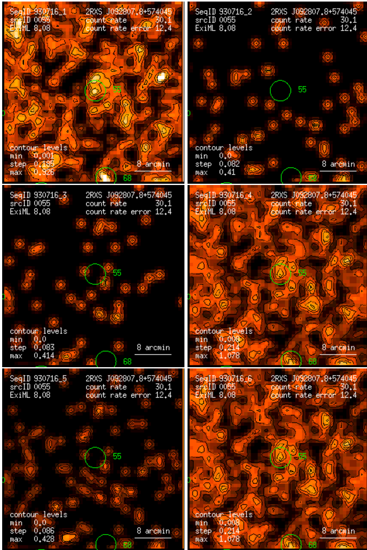
Figure 55: RASS 930716: detection 0055: band rate images, Gaussian filter: (1) PSPC channels 11 – 41, (2) 52 – 90, (3) 91 – 201, (4) 11 – 235, (5) 52 – 201, (6) 11 – 201. Broad band rates in counts/ks. Band rate contour levels in counts/ks/arcmin 2 .
