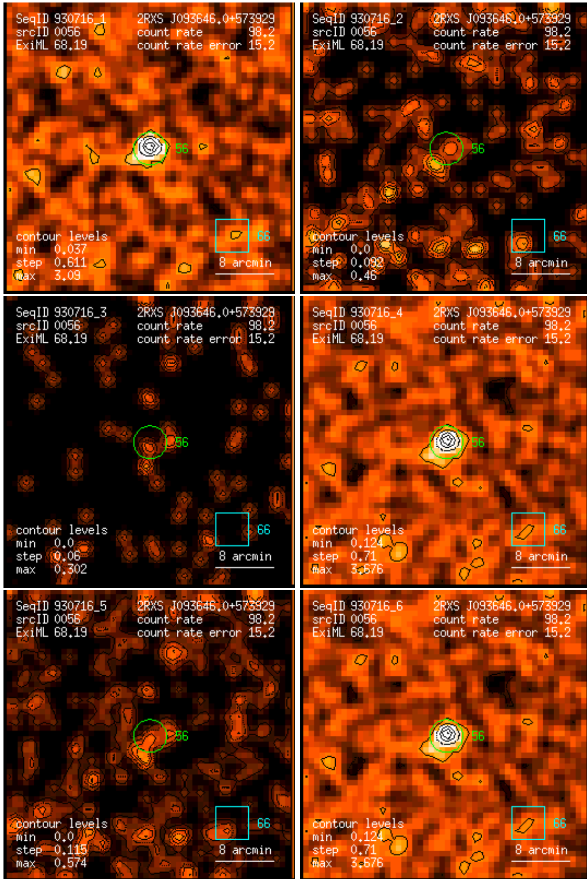
Figure 56: RASS 930716: detection 0056: band rate images, Gaussian filter: (1) PSPC channels 11 – 41, (2) 52 – 90, (3) 91 – 201, (4) 11 – 235, (5) 52 – 201, (6) 11 – 201. Broad band rates in counts/ks. Band rate contour levels in counts/ks/arcmin 2 .
