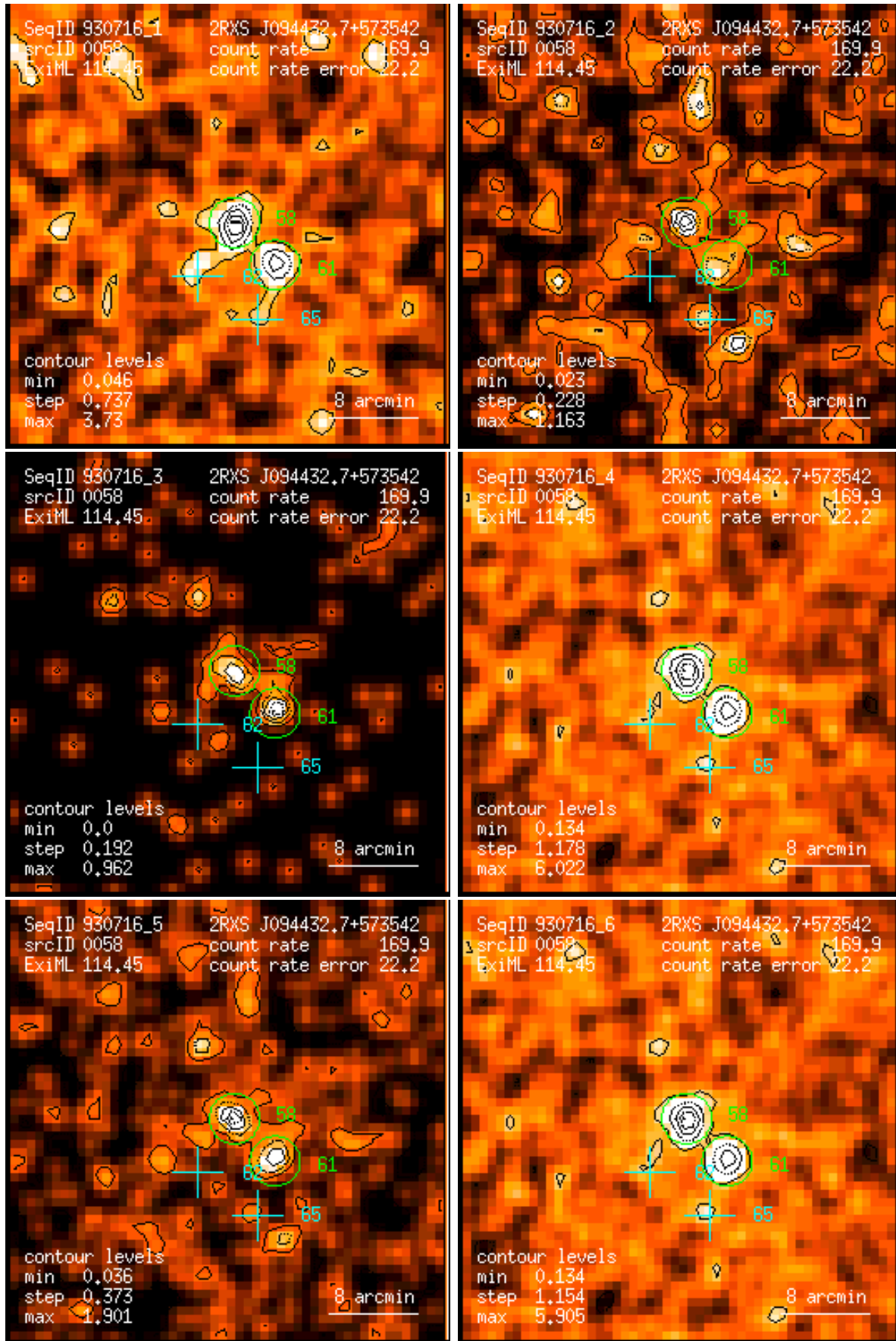
Figure 58: RASS 930716: detection 0058: band rate images, Gaussian filter: (1) PSPC channels 11 – 41, (2) 52 – 90, (3) 91 – 201, (4) 11 – 235, (5) 52 – 201, (6) 11 – 201. Broad band rates in counts/ks. Band rate contour levels in counts/ks/arcmin 2 .
