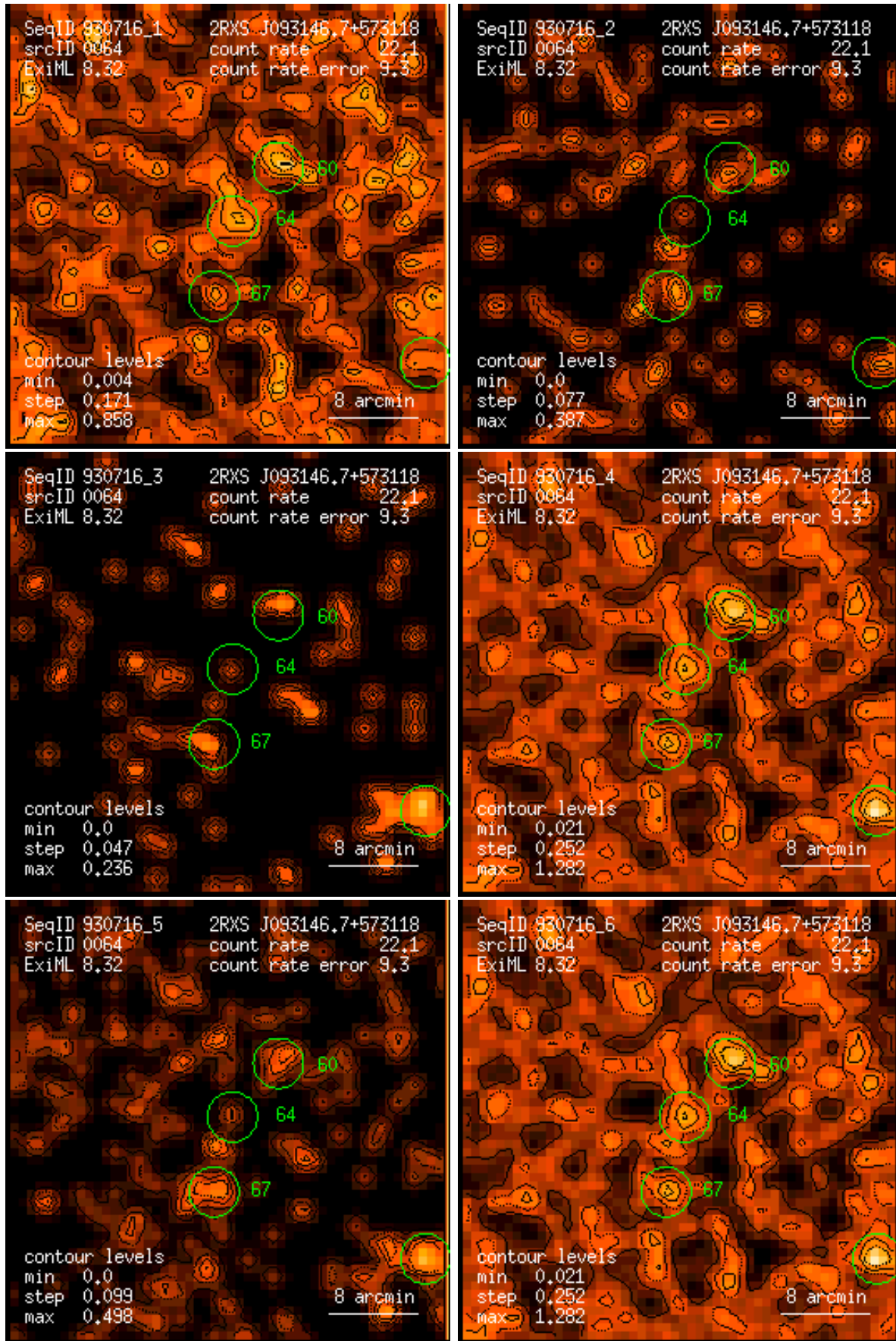
Figure 64: RASS 930716: detection 0064: band rate images, Gaussian filter: (1) PSPC channels 11 – 41, (2) 52 – 90, (3) 91 – 201, (4) 11 – 235, (5) 52 – 201, (6) 11 – 201. Broad band rates in counts/ks. Band rate contour levels in counts/ks/arcmin 2 .
