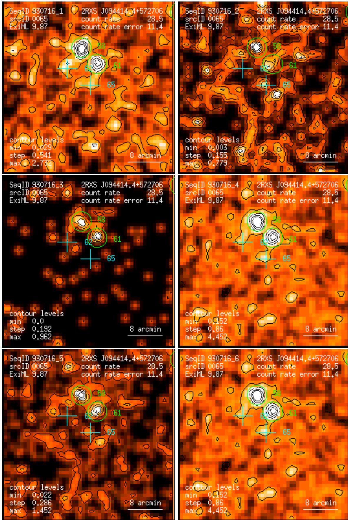
Figure 65: RASS 930716: detection 0065: band rate images, Gaussian filter: (1) PSPC channels 11 – 41, (2) 52 – 90, (3) 91 – 201, (4) 11 – 235, (5) 52 – 201, (6) 11 – 201. Broad band rates in counts/ks. Band rate contour levels in counts/ks/arcmin 2 .
