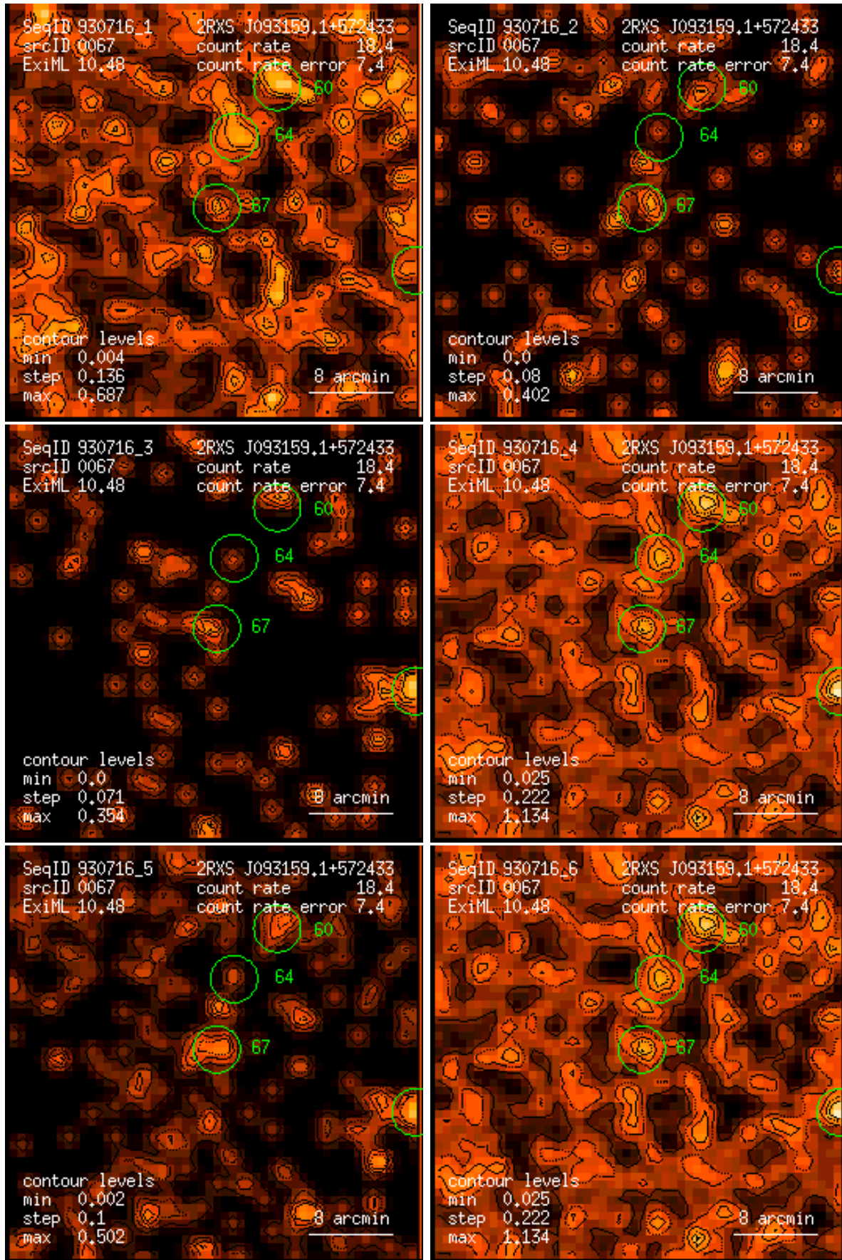
Figure 67: RASS 930716: detection 0067: band rate images, Gaussian filter: (1) PSPC channels 11 – 41, (2) 52 – 90, (3) 91 – 201, (4) 11 – 235, (5) 52 – 201, (6) 11 – 201. Broad band rates in counts/ks. Band rate contour levels in counts/ks/arcmin 2 .
