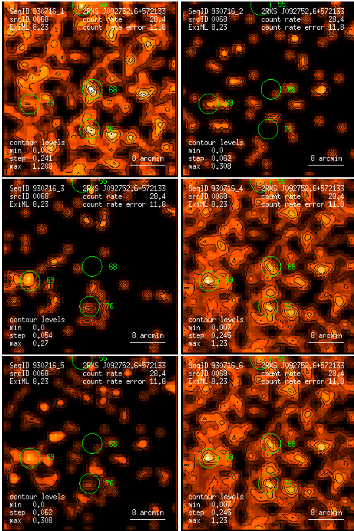
Figure 68: RASS 930716: detection 0068: band rate images, Gaussian filter: (1) PSPC channels 11 – 41, (2) 52 – 90, (3) 91 – 201, (4) 11 – 235, (5) 52 – 201, (6) 11 – 201. Broad band rates in counts/ks. Band rate contour levels in counts/ks/arcmin 2 .
