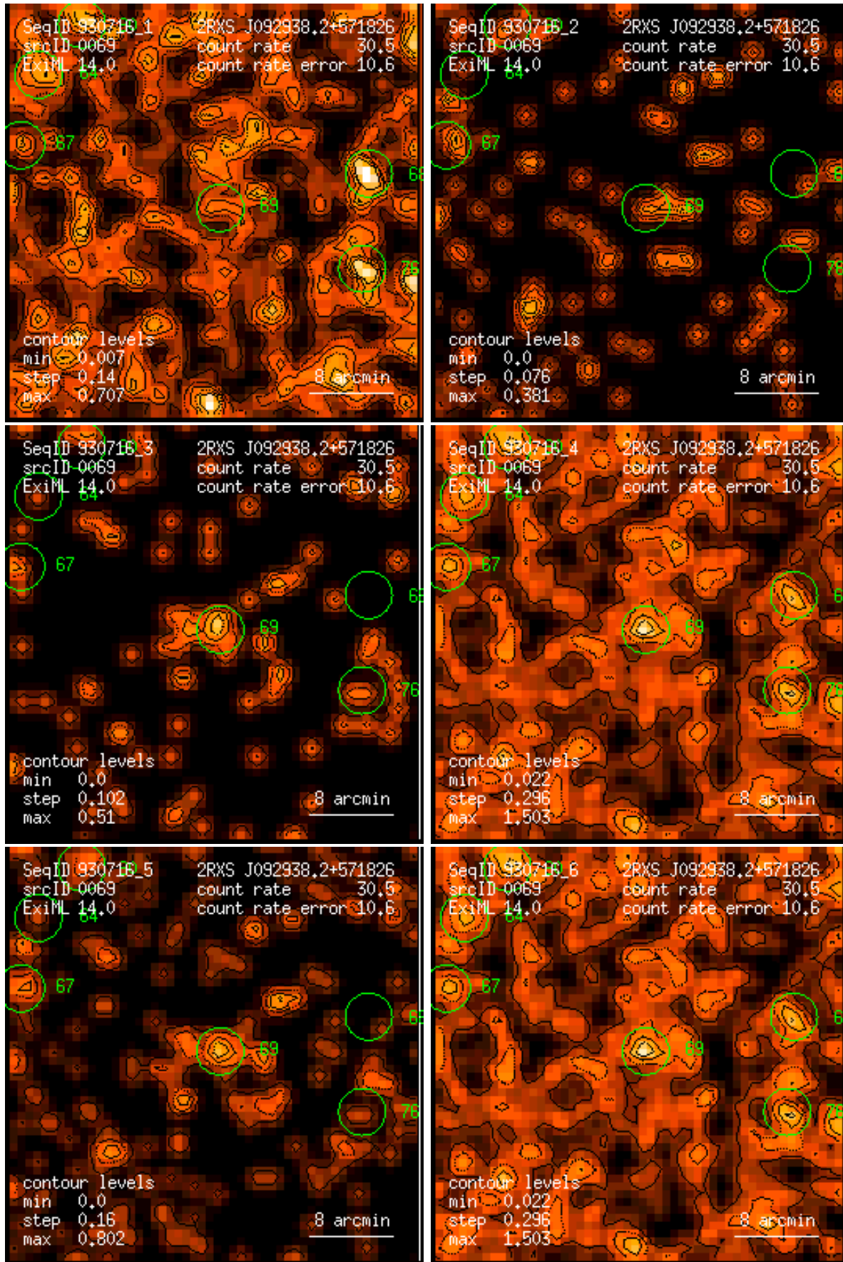
Figure 69: RASS 930716: detection 0069: band rate images, Gaussian filter: (1) PSPC channels 11 – 41, (2) 52 – 90, (3) 91 – 201, (4) 11 – 235, (5) 52 – 201, (6) 11 – 201. Broad band rates in counts/ks. Band rate contour levels in counts/ks/arcmin 2 .
