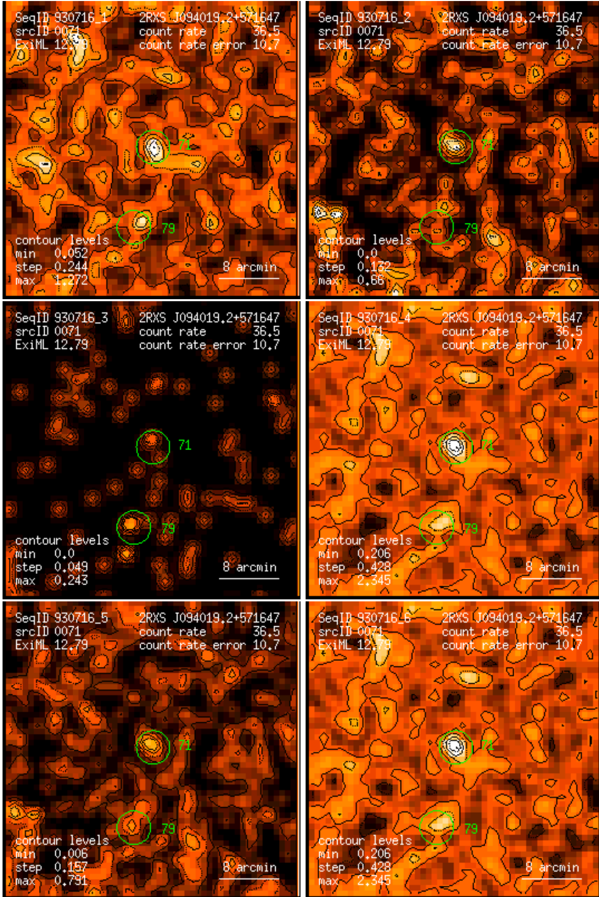
Figure 71: RASS 930716: detection 0071: band rate images, Gaussian filter: (1) PSPC channels 11 – 41, (2) 52 – 90, (3) 91 – 201, (4) 11 – 235, (5) 52 – 201, (6) 11 – 201. Broad band rates in counts/ks. Band rate contour levels in counts/ks/arcmin 2 .
