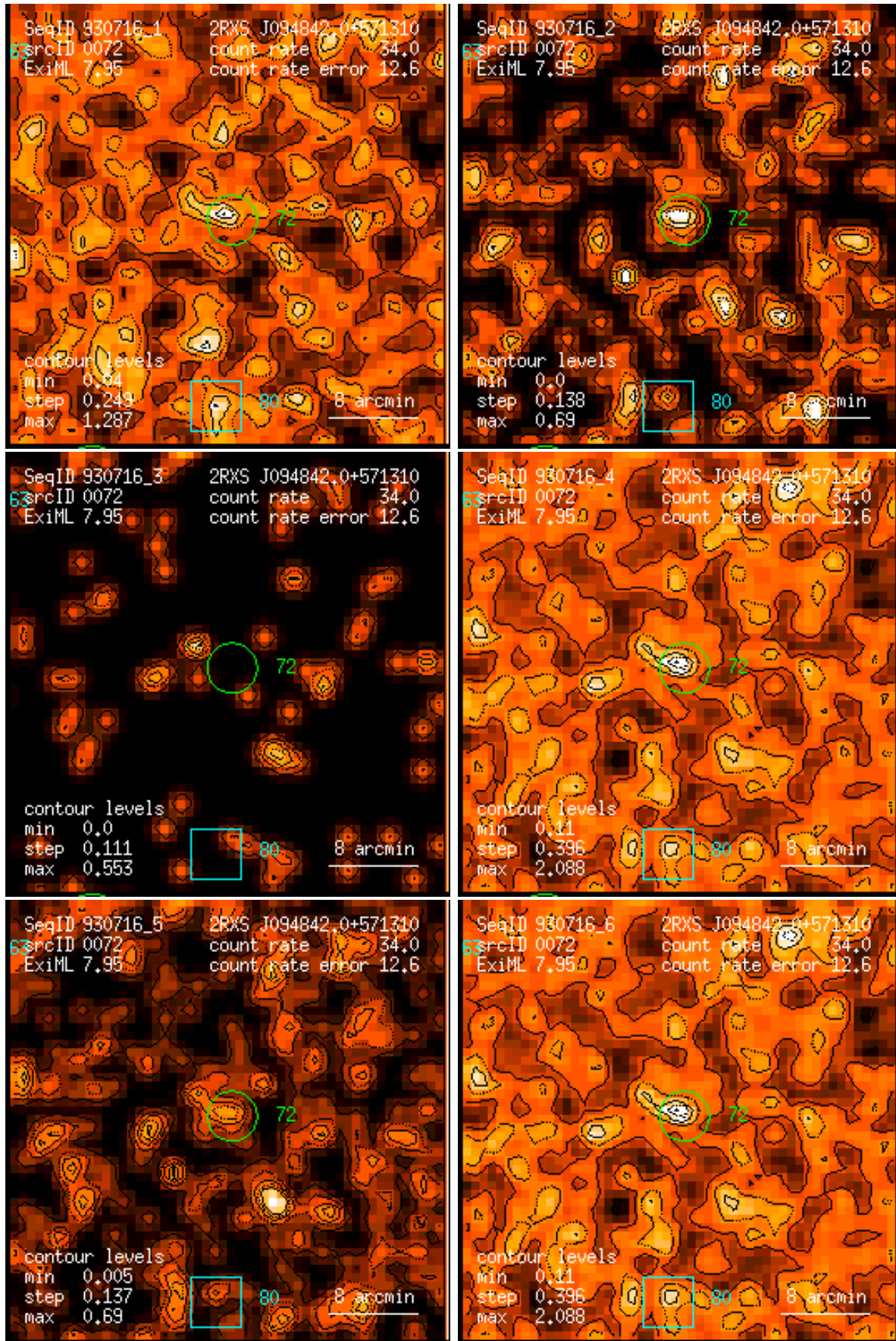
Figure 72: RASS 930716: detection 0072: band rate images, Gaussian filter: (1) PSPC channels 11 – 41, (2) 52 – 90, (3) 91 – 201, (4) 11 – 235, (5) 52 – 201, (6) 11 – 201. Broad band rates in counts/ks. Band rate contour levels in counts/ks/arcmin 2 .
