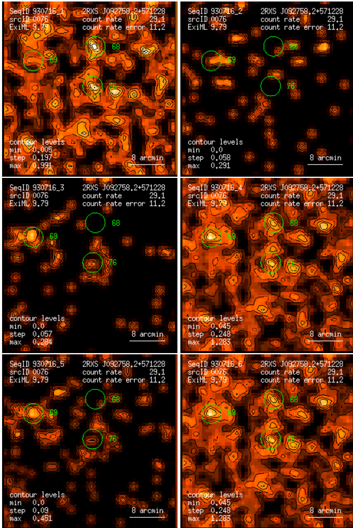
Figure 76: RASS 930716: detection 0076: band rate images, Gaussian filter: (1) PSPC channels 11 – 41, (2) 52 – 90, (3) 91 – 201, (4) 11 – 235, (5) 52 – 201, (6) 11 – 201. Broad band rates in counts/ks. Band rate contour levels in counts/ks/arcmin 2 .
