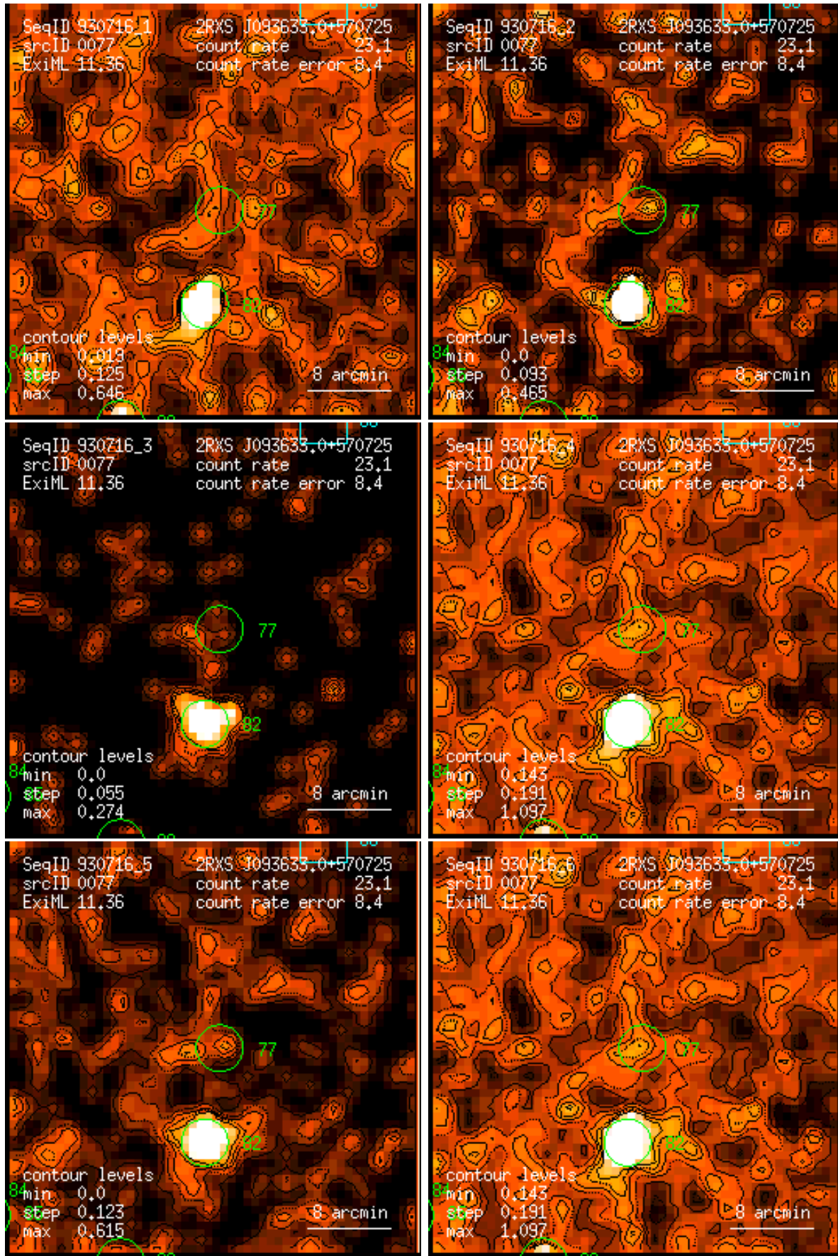
Figure 77: RASS 930716: detection 0077: band rate images, Gaussian filter: (1) PSPC channels 11 – 41, (2) 52 – 90, (3) 91 – 201, (4) 11 – 235, (5) 52 – 201, (6) 11 – 201. Broad band rates in counts/ks. Band rate contour levels in counts/ks/arcmin 2 .
