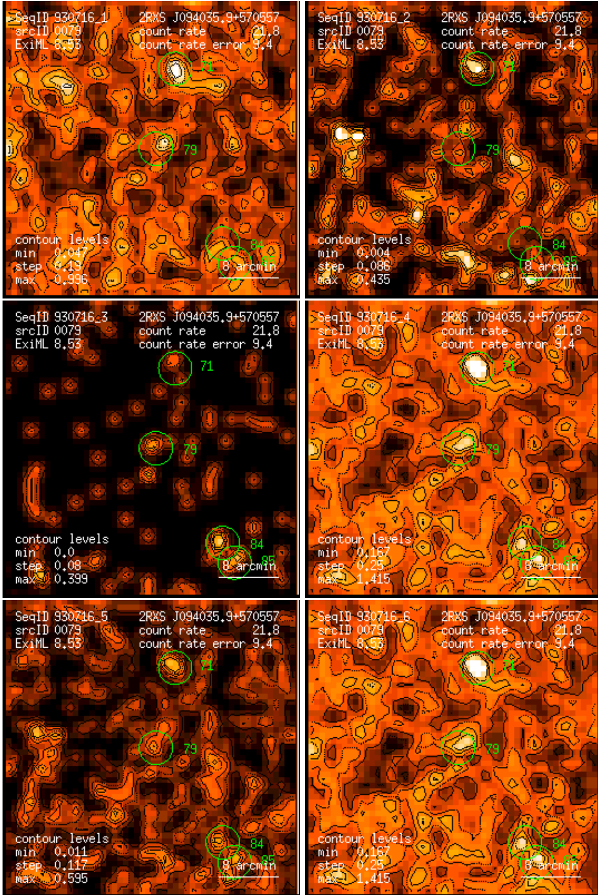
Figure 79: RASS 930716: detection 0079: band rate images, Gaussian filter: (1) PSPC channels 11 – 41, (2) 52 – 90, (3) 91 – 201, (4) 11 – 235, (5) 52 – 201, (6) 11 – 201. Broad band rates in counts/ks. Band rate contour levels in counts/ks/arcmin 2 .
