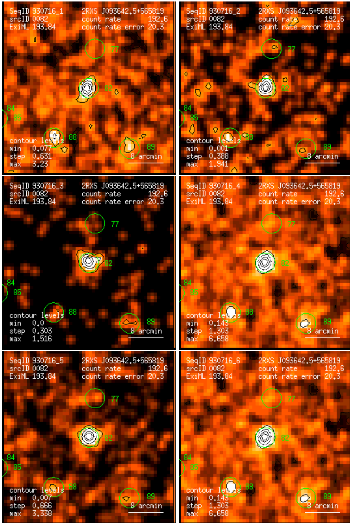
Figure 82: RASS 930716: detection 0082: band rate images, Gaussian filter: (1) PSPC channels 11 – 41, (2) 52 – 90, (3) 91 – 201, (4) 11 – 235, (5) 52 – 201, (6) 11 – 201. Broad band rates in counts/ks. Band rate contour levels in counts/ks/arcmin 2 .
