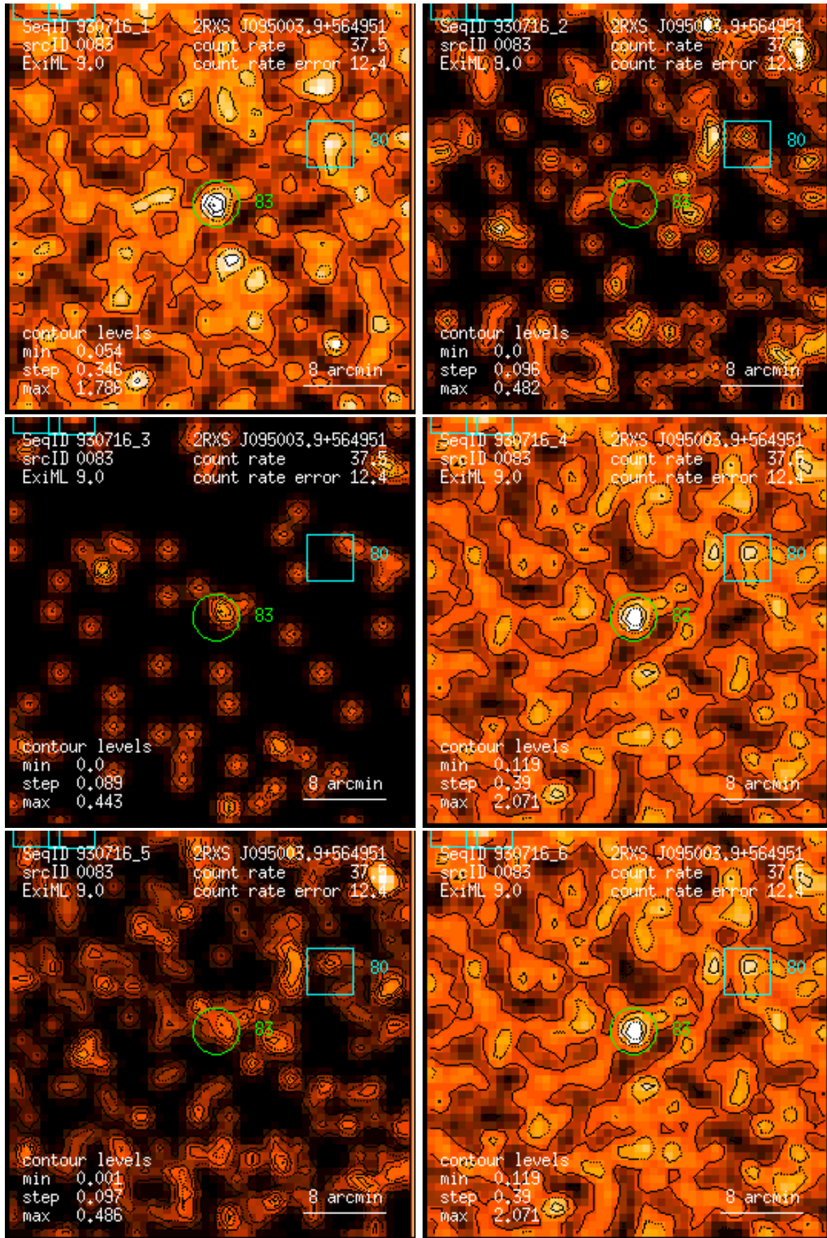
Figure 83: RASS 930716: detection 0083: band rate images, Gaussian filter: (1) PSPC channels 11 – 41, (2) 52 – 90, (3) 91 – 201, (4) 11 – 235, (5) 52 – 201, (6) 11 – 201. Broad band rates in counts/ks. Band rate contour levels in counts/ks/arcmin 2 .
