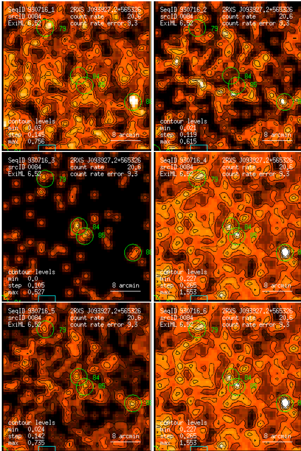
Figure 84: RASS 930716: detection 0084: band rate images, Gaussian filter: (1) PSPC channels 11 – 41, (2) 52 – 90, (3) 91 – 201, (4) 11 – 235, (5) 52 – 201, (6) 11 – 201. Broad band rates in counts/ks. Band rate contour levels in counts/ks/arcmin 2 .
