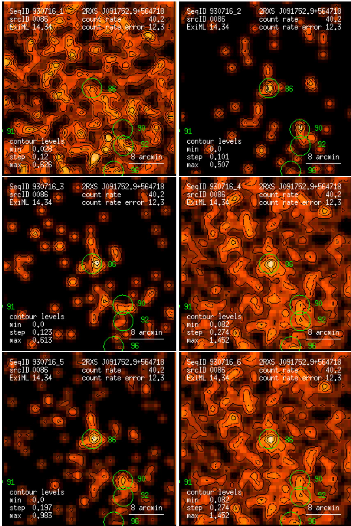
Figure 86: RASS 930716: detection 0086: band rate images, Gaussian filter: (1) PSPC channels 11 – 41, (2) 52 – 90, (3) 91 – 201, (4) 11 – 235, (5) 52 – 201, (6) 11 – 201. Broad band rates in counts/ks. Band rate contour levels in counts/ks/arcmin 2 .
