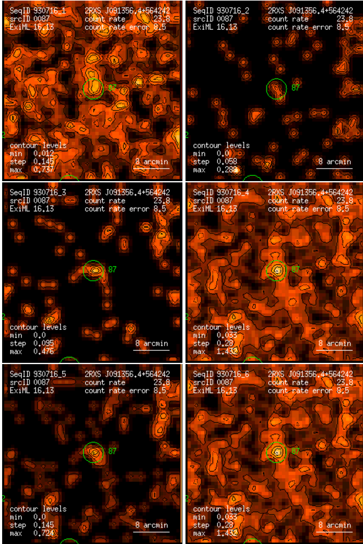
Figure 87: RASS 930716: detection 0087: band rate images, Gaussian filter: (1) PSPC channels 11 – 41, (2) 52 – 90, (3) 91 – 201, (4) 11 – 235, (5) 52 – 201, (6) 11 – 201. Broad band rates in counts/ks. Band rate contour levels in counts/ks/arcmin 2 .
