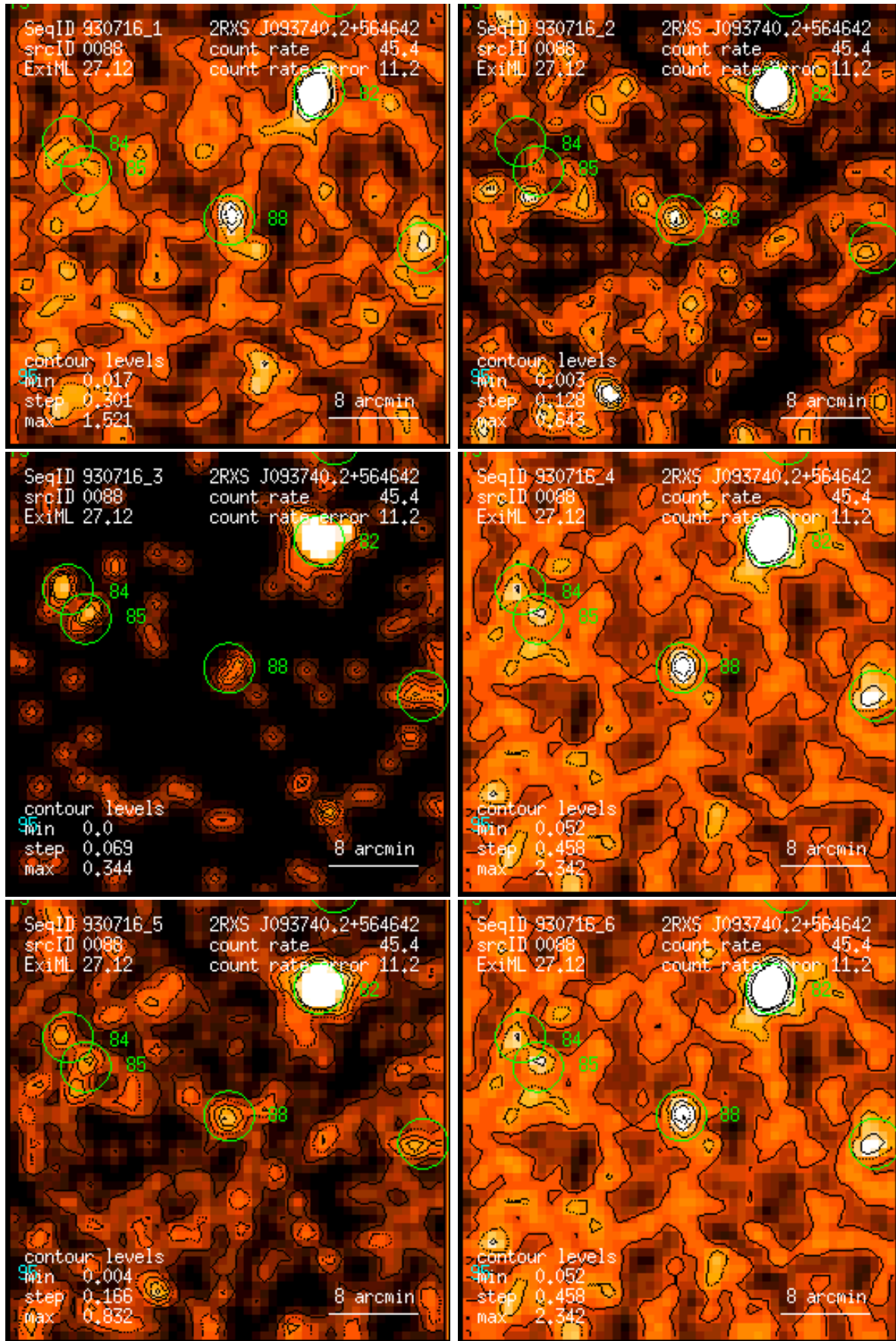
Figure 88: RASS 930716: detection 0088: band rate images, Gaussian filter: (1) PSPC channels 11 – 41, (2) 52 – 90, (3) 91 – 201, (4) 11 – 235, (5) 52 – 201, (6) 11 – 201. Broad band rates in counts/ks. Band rate contour levels in counts/ks/arcmin 2 .
