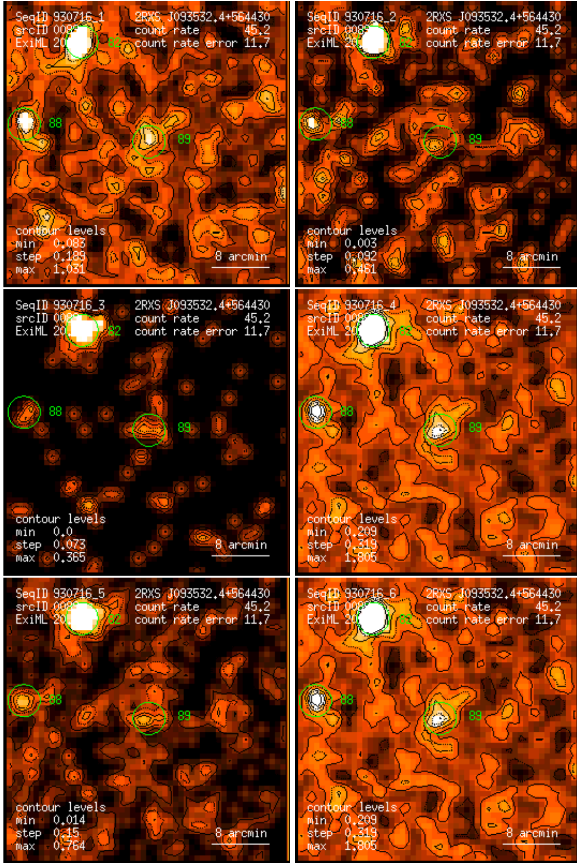
Figure 89: RASS 930716: detection 0089: band rate images, Gaussian filter: (1) PSPC channels 11 – 41, (2) 52 – 90, (3) 91 – 201, (4) 11 – 235, (5) 52 – 201, (6) 11 – 201. Broad band rates in counts/ks. Band rate contour levels in counts/ks/arcmin 2 .
