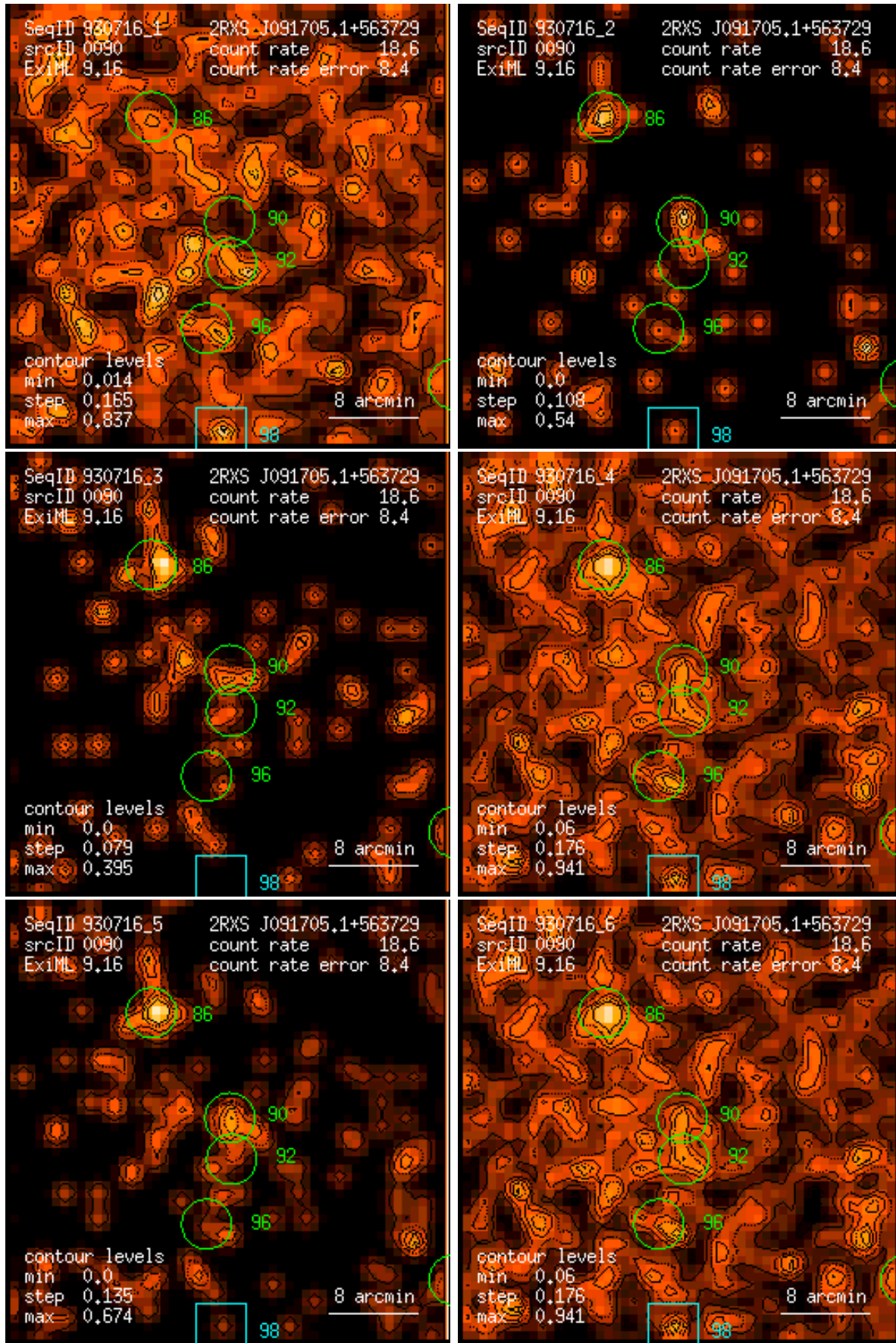
Figure 90: RASS 930716: detection 0090: band rate images, Gaussian filter: (1) PSPC channels 11 – 41, (2) 52 – 90, (3) 91 – 201, (4) 11 – 235, (5) 52 – 201, (6) 11 – 201. Broad band rates in counts/ks. Band rate contour levels in counts/ks/arcmin 2 .
