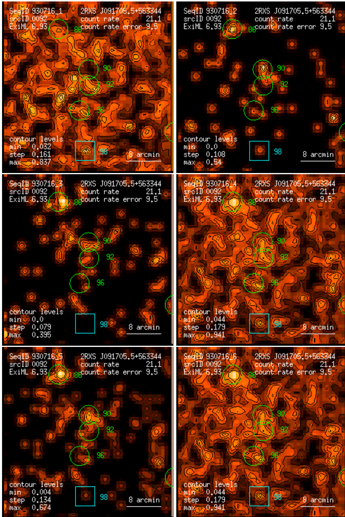
Figure 92: RASS 930716: detection 0092: band rate images, Gaussian filter: (1) PSPC channels 11 – 41, (2) 52 – 90, (3) 91 – 201, (4) 11 – 235, (5) 52 – 201, (6) 11 – 201. Broad band rates in counts/ks. Band rate contour levels in counts/ks/arcmin 2 .
