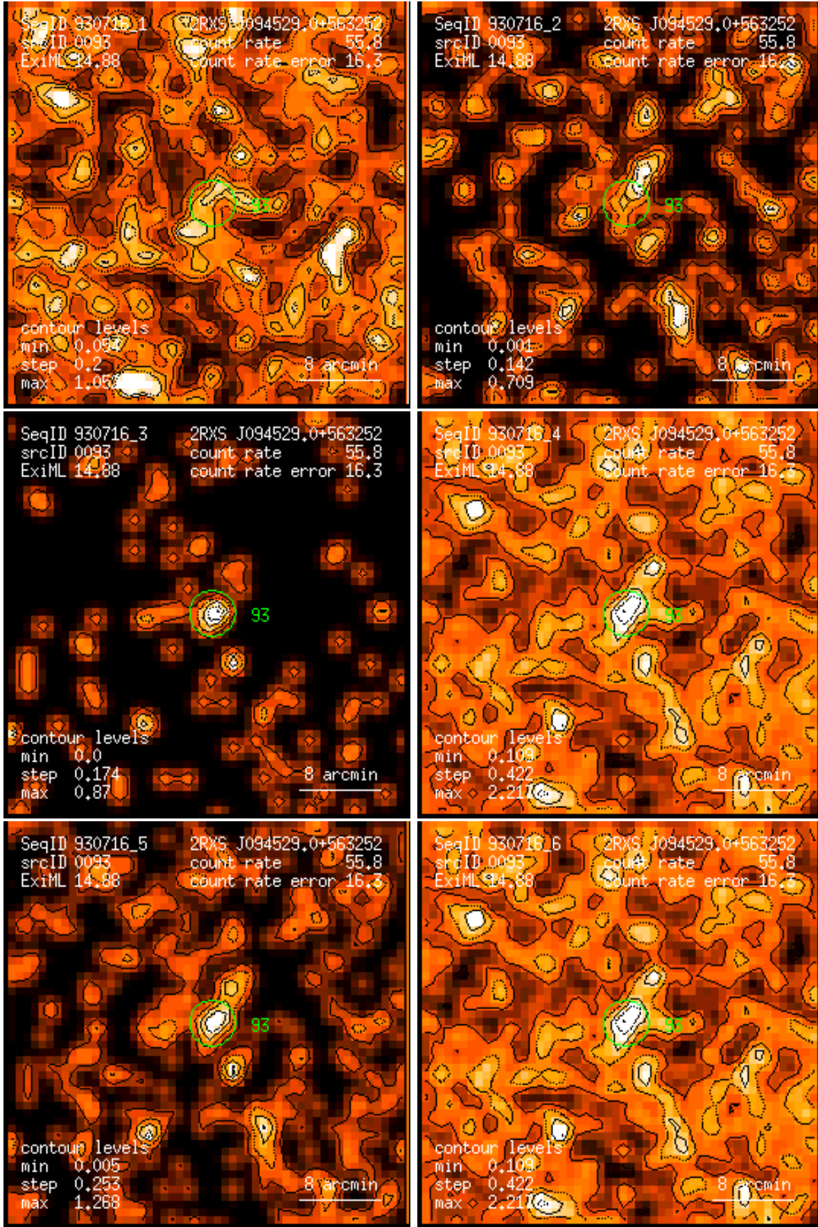
Figure 93: RASS 930716: detection 0093: band rate images, Gaussian filter: (1) PSPC channels 11 – 41, (2) 52 – 90, (3) 91 – 201, (4) 11 – 235, (5) 52 – 201, (6) 11 – 201. Broad band rates in counts/ks. Band rate contour levels in counts/ks/arcmin 2 .
