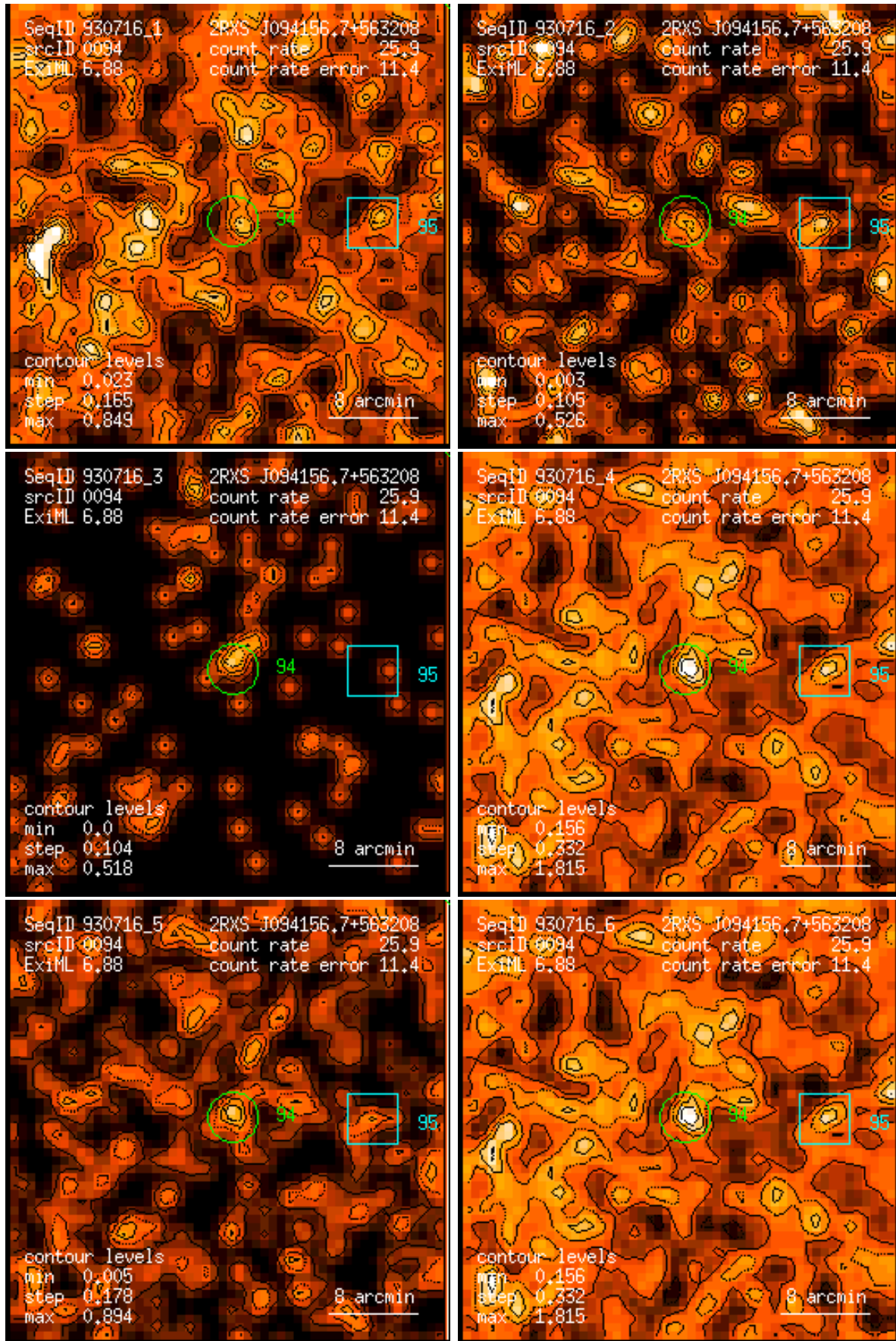
Figure 94: RASS 930716: detection 0094: band rate images, Gaussian filter: (1) PSPC channels 11 – 41, (2) 52 – 90, (3) 91 – 201, (4) 11 – 235, (5) 52 – 201, (6) 11 – 201. Broad band rates in counts/ks. Band rate contour levels in counts/ks/arcmin 2 .
