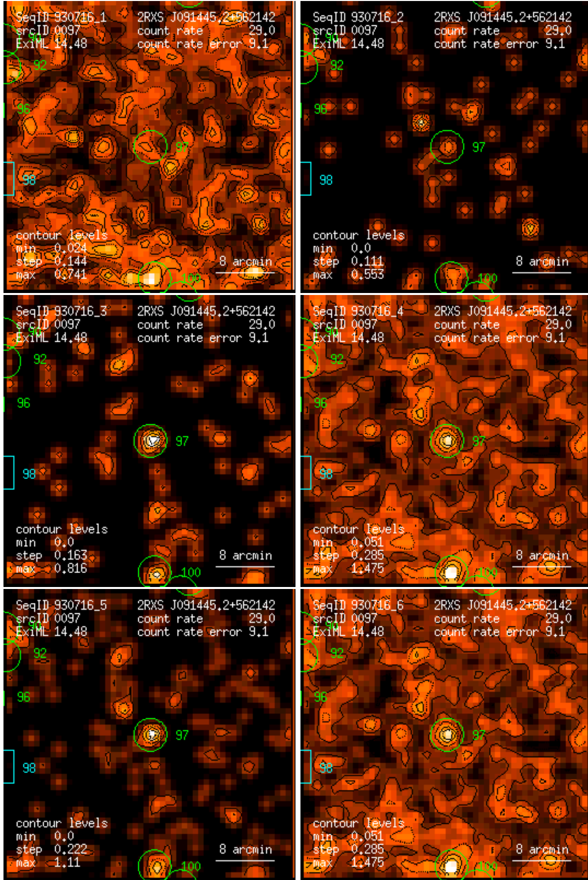
Figure 97: RASS 930716: detection 0097: band rate images, Gaussian filter: (1) PSPC channels 11 – 41, (2) 52 – 90, (3) 91 – 201, (4) 11 – 235, (5) 52 – 201, (6) 11 – 201. Broad band rates in counts/ks. Band rate contour levels in counts/ks/arcmin 2 .
